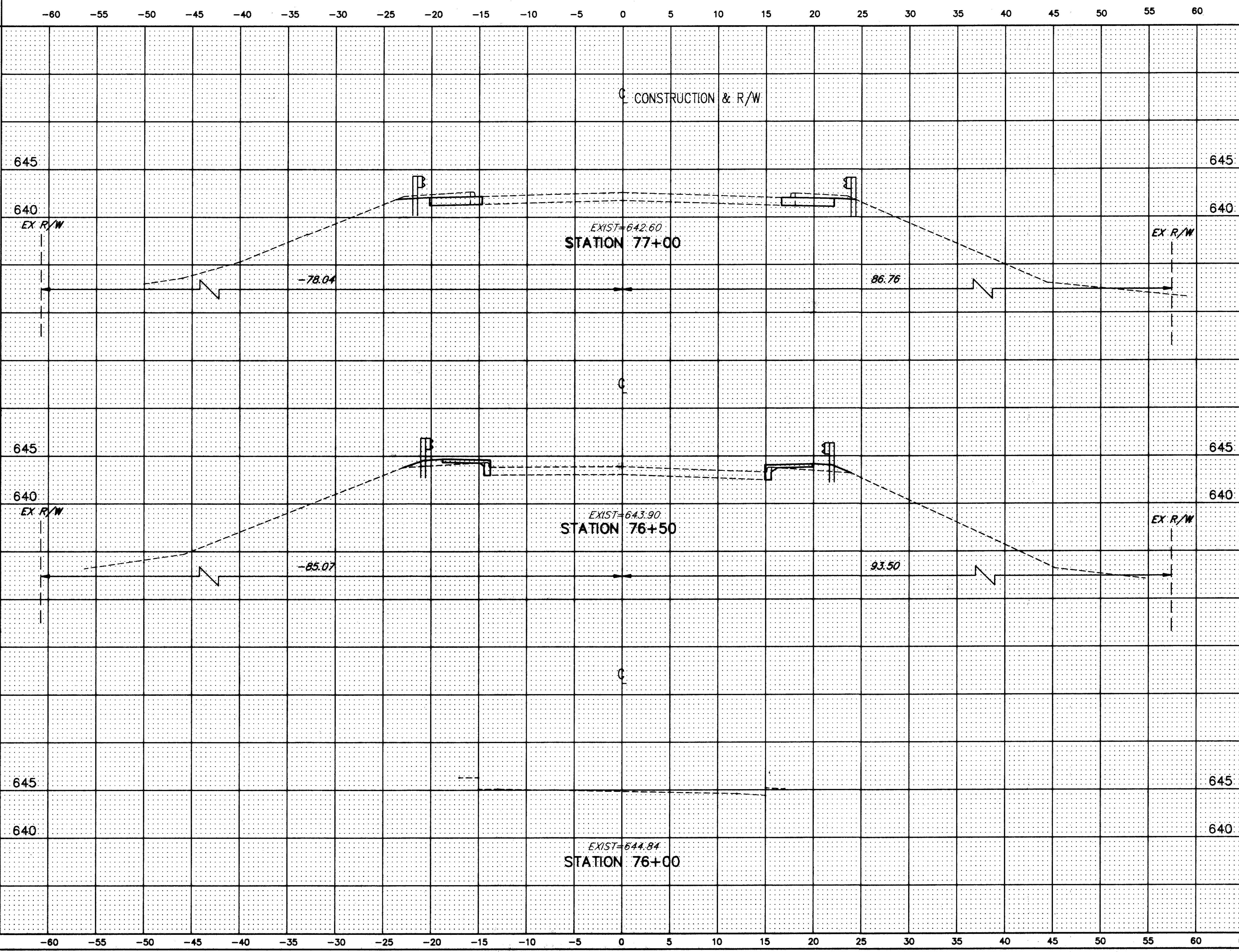
HOPKINS ROAD CROSS-SECTIONS STA. 76+00 TO STA. 77+00
