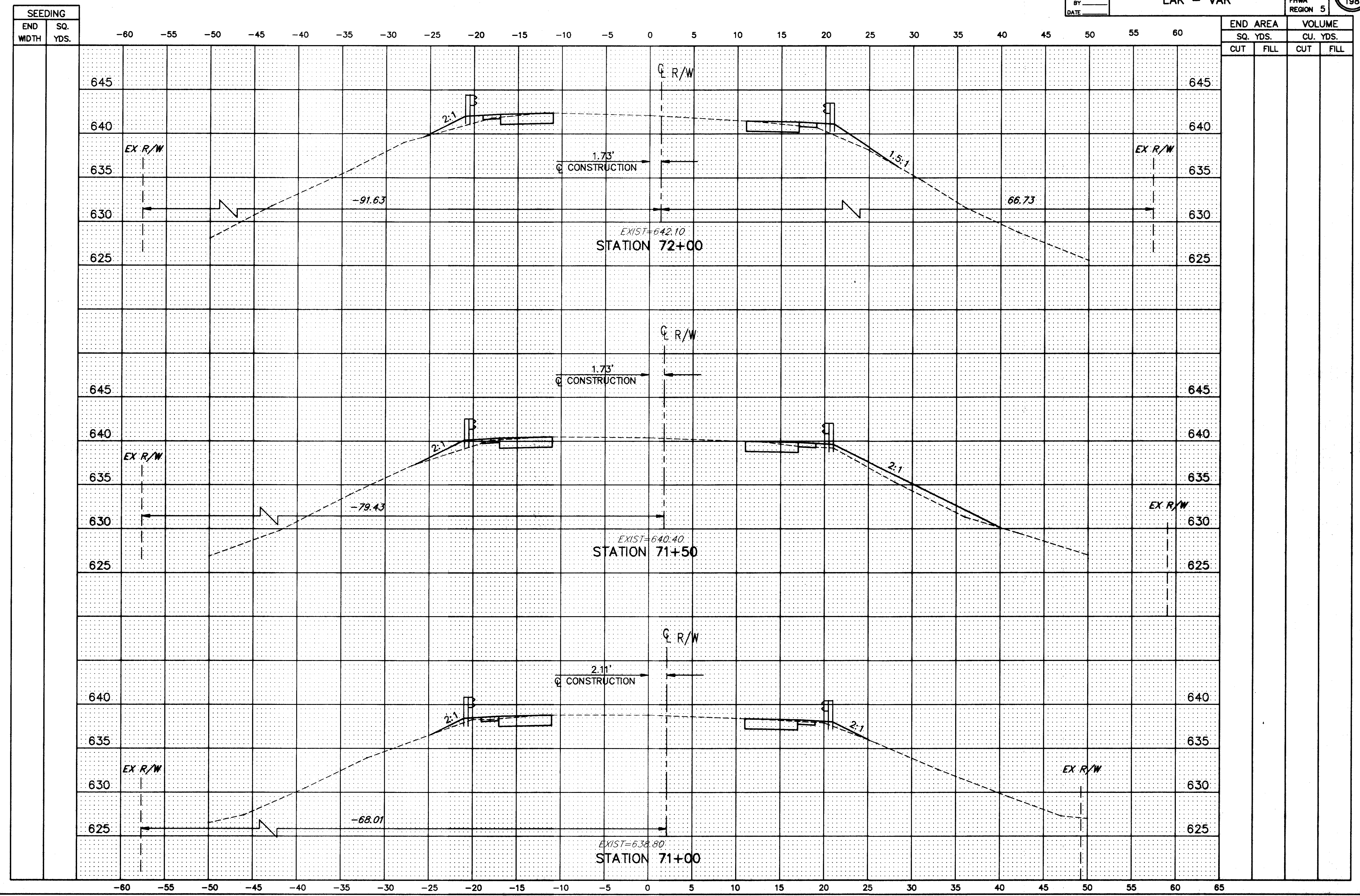
HOPKINS ROAD CROSS-SECTIONS STA. 71+00 TO STA. 72+00
