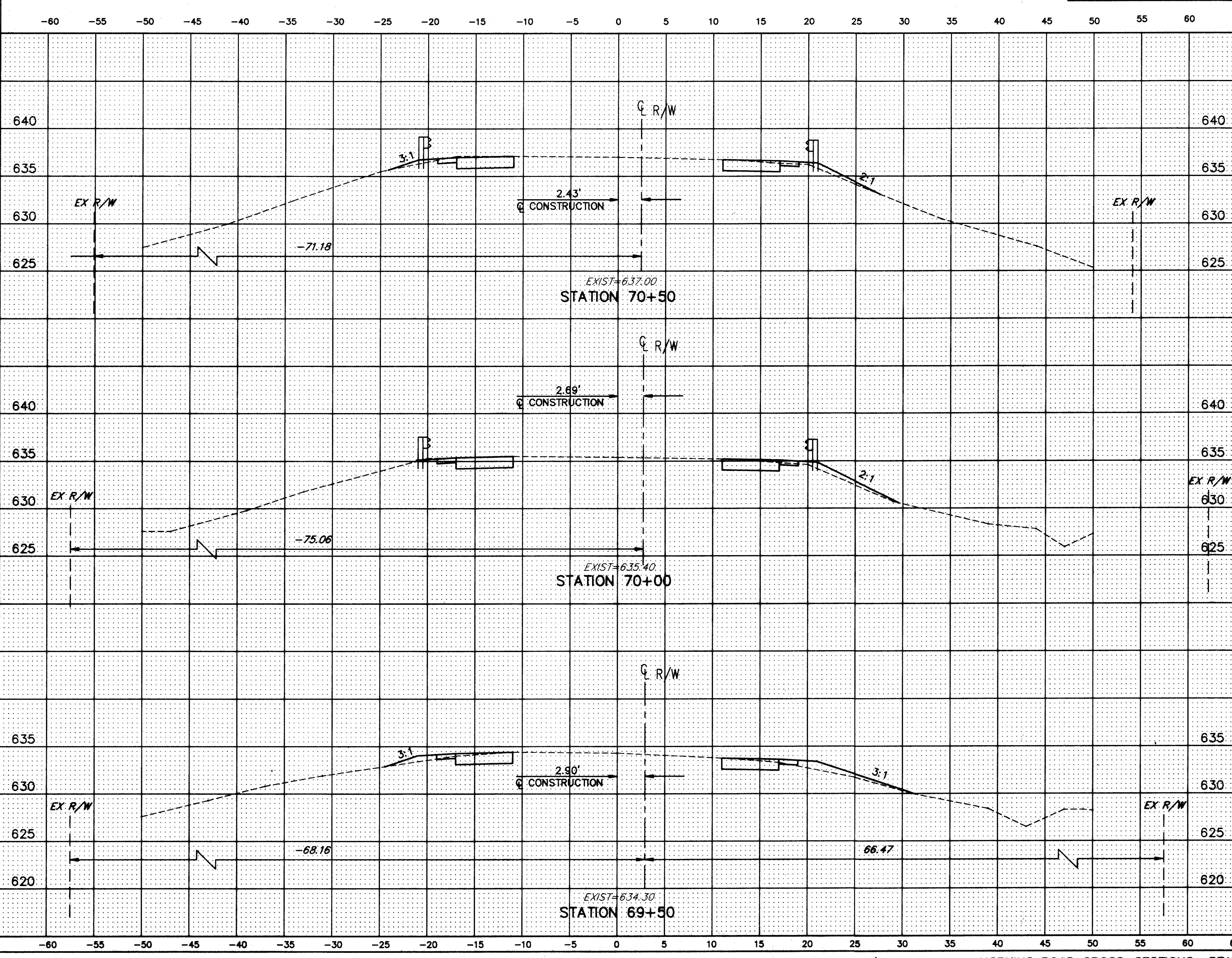
HOPKINS ROAD CROSS-SECTIONS STA. 69+50 TO STA. 70+50
