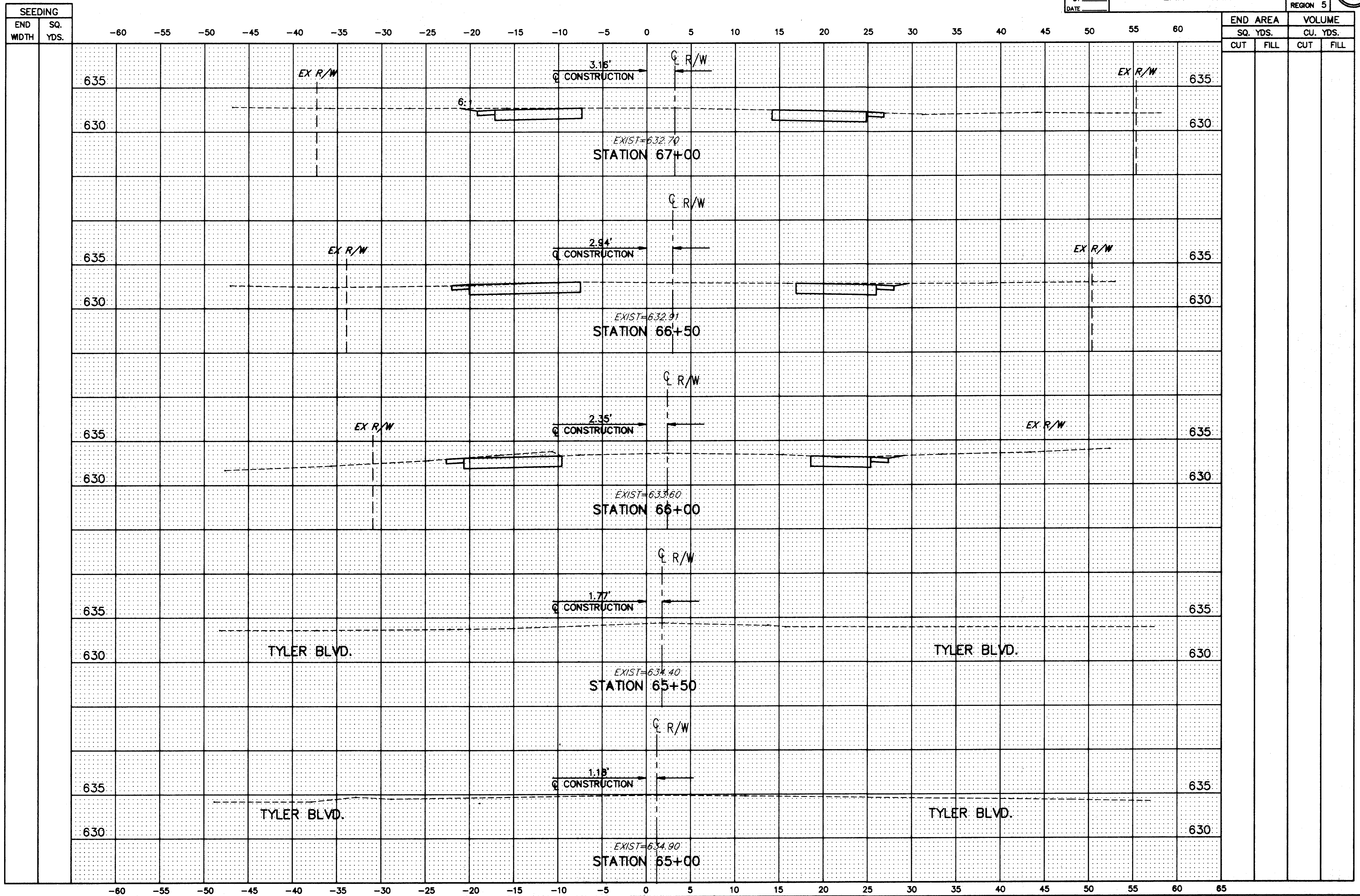
HOPKINS ROAD CROSS-SECTIONS STA. 65+00 TO STA. 67+00
