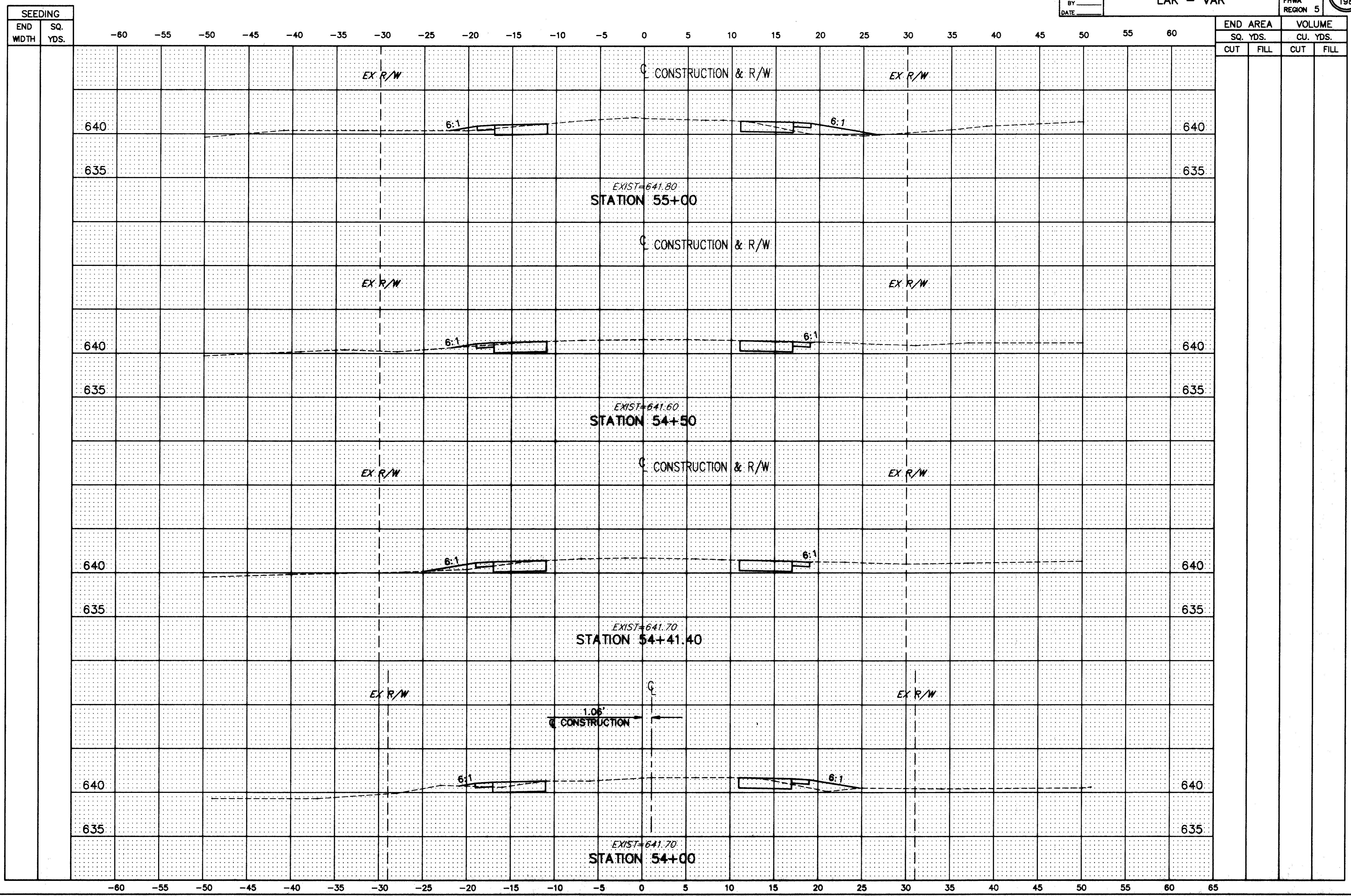
HOPKINS ROAD CROSS-SECTIONS STA. 54+00 TO STA. 55+00
