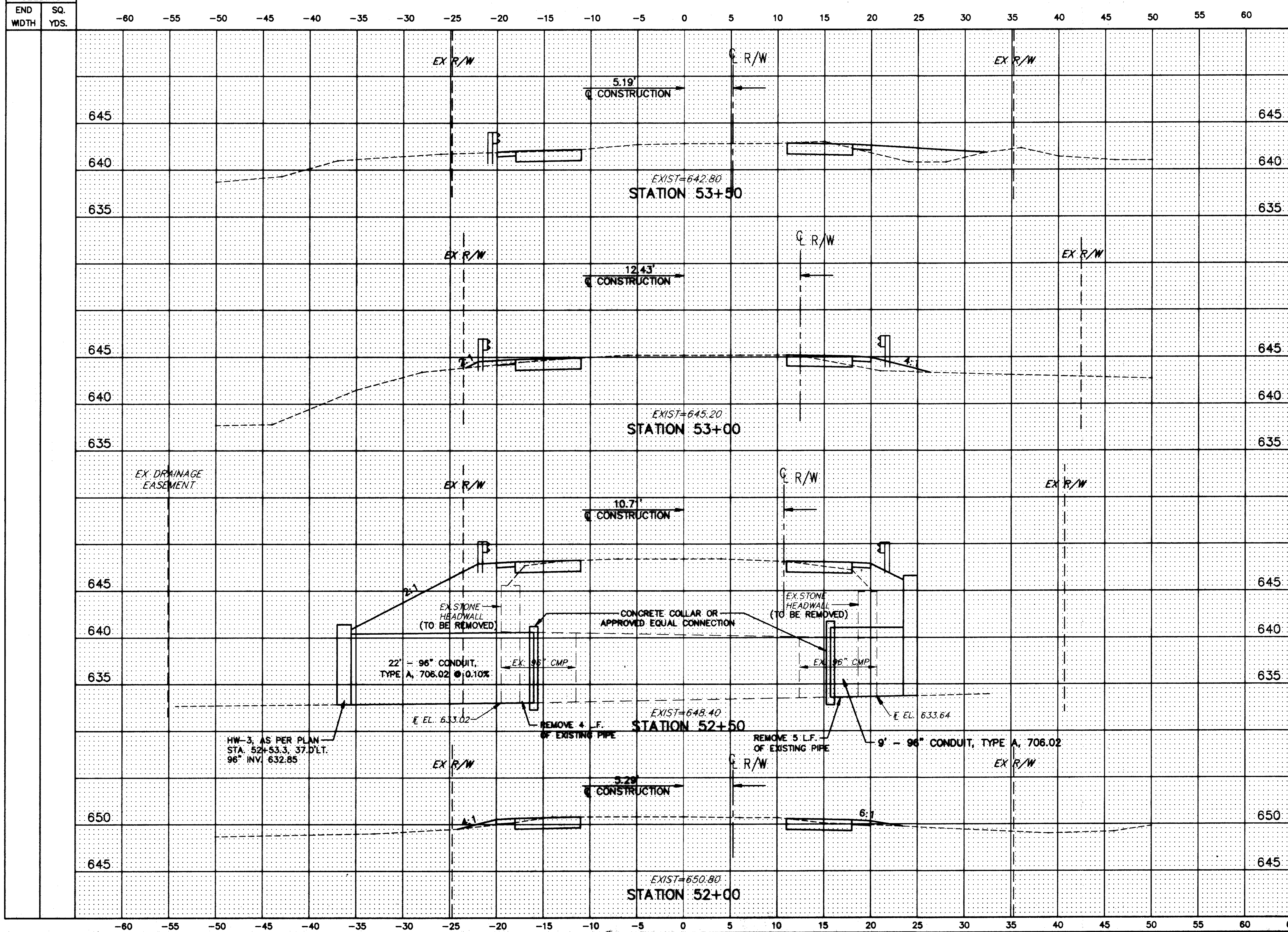
HOPKINS ROAD CROSS-SECTIONS STA. 52+00 TO STA. 53+50
