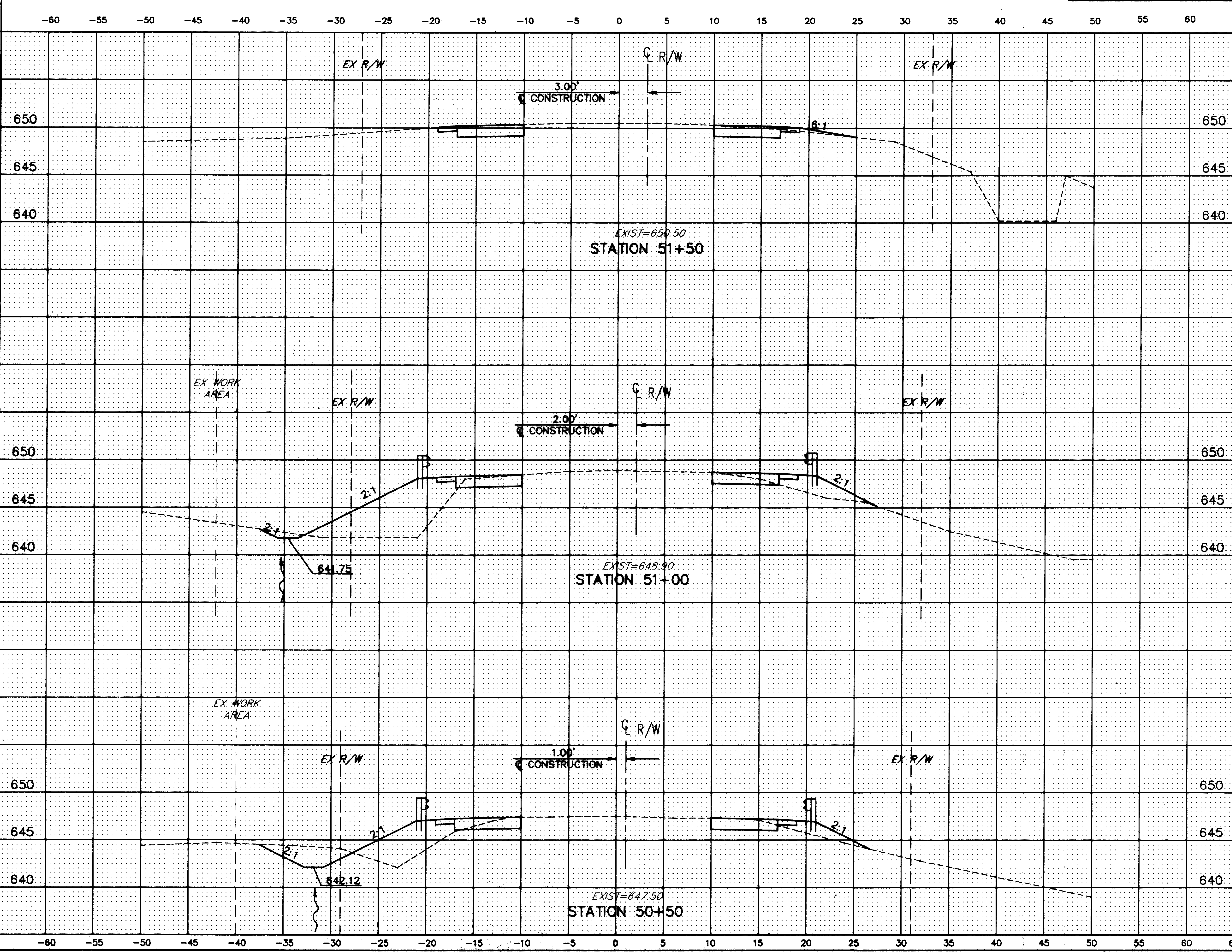
HOPKINS ROAD CROSS-SECTIONS STA. 50+50 TO STA. 51+50
