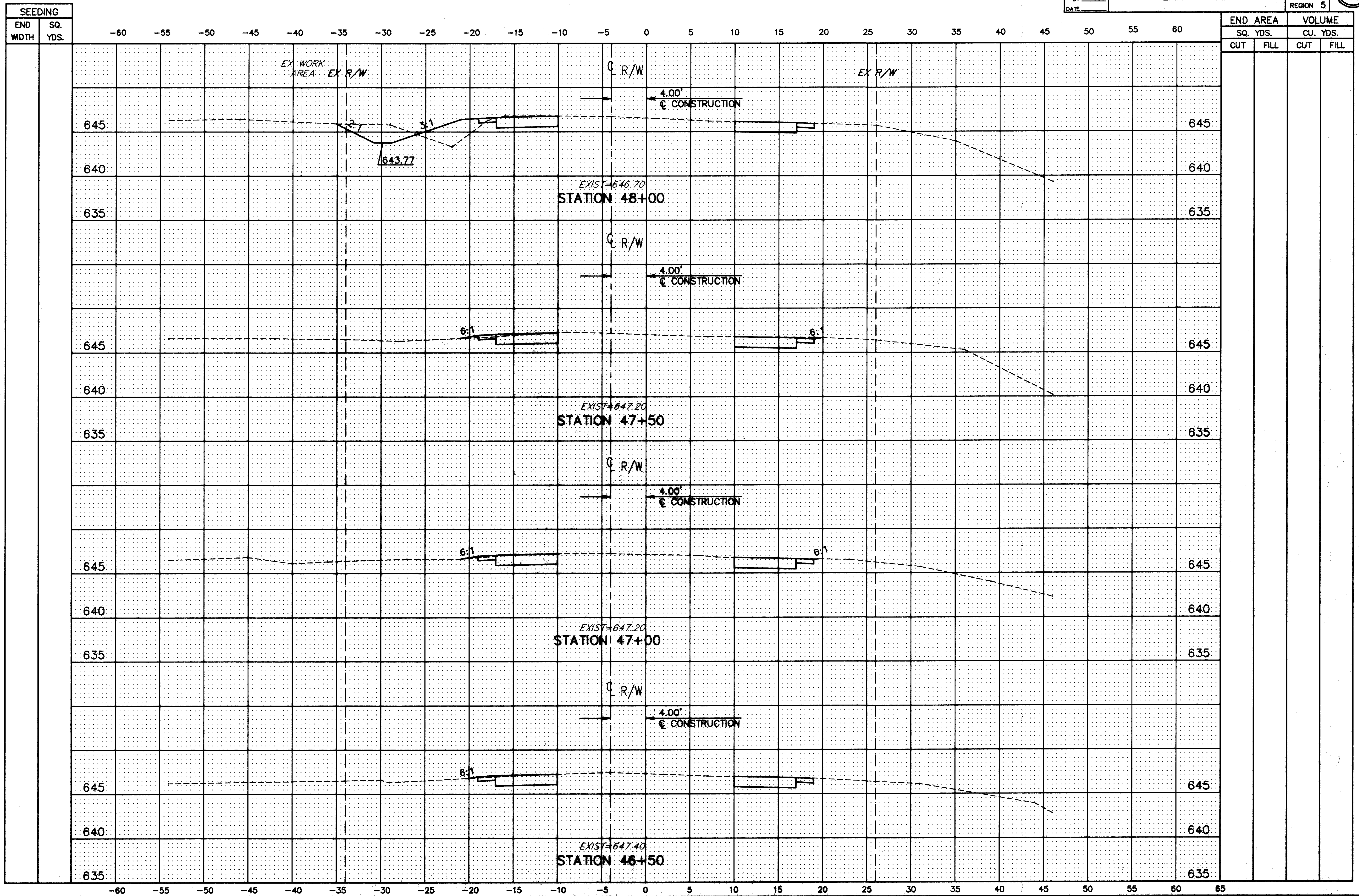
HOPKINS ROAD CROSS-SECTIONS STA. 46+50 TO STA. 48+00
