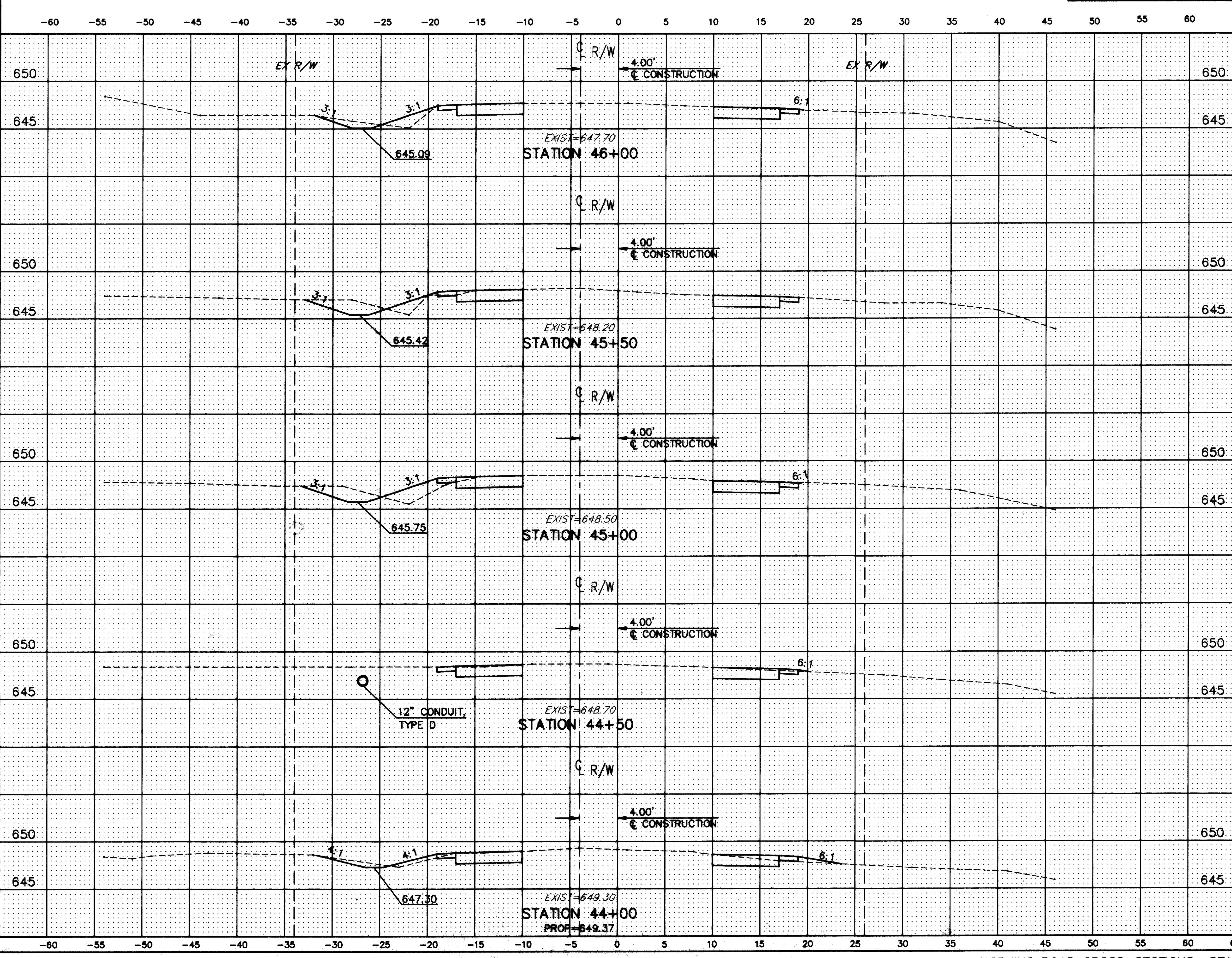
HOPKINS ROAD CROSS-SECTIONS STA. 44+00 TO STA. 46+00
