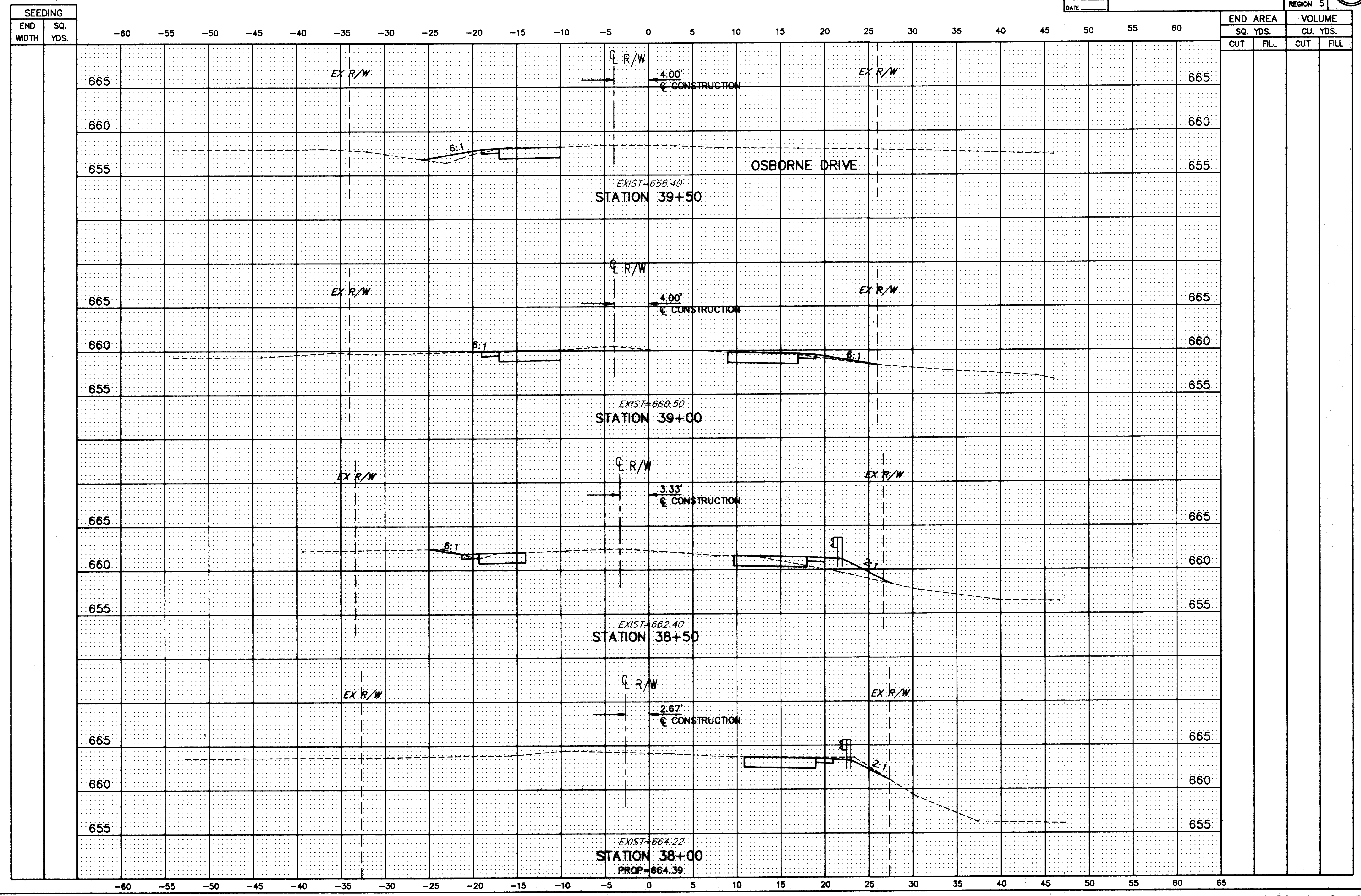
HOPKINS ROAD CROSS-SECTIONS STA. 38+00 TO STA. 39+50
