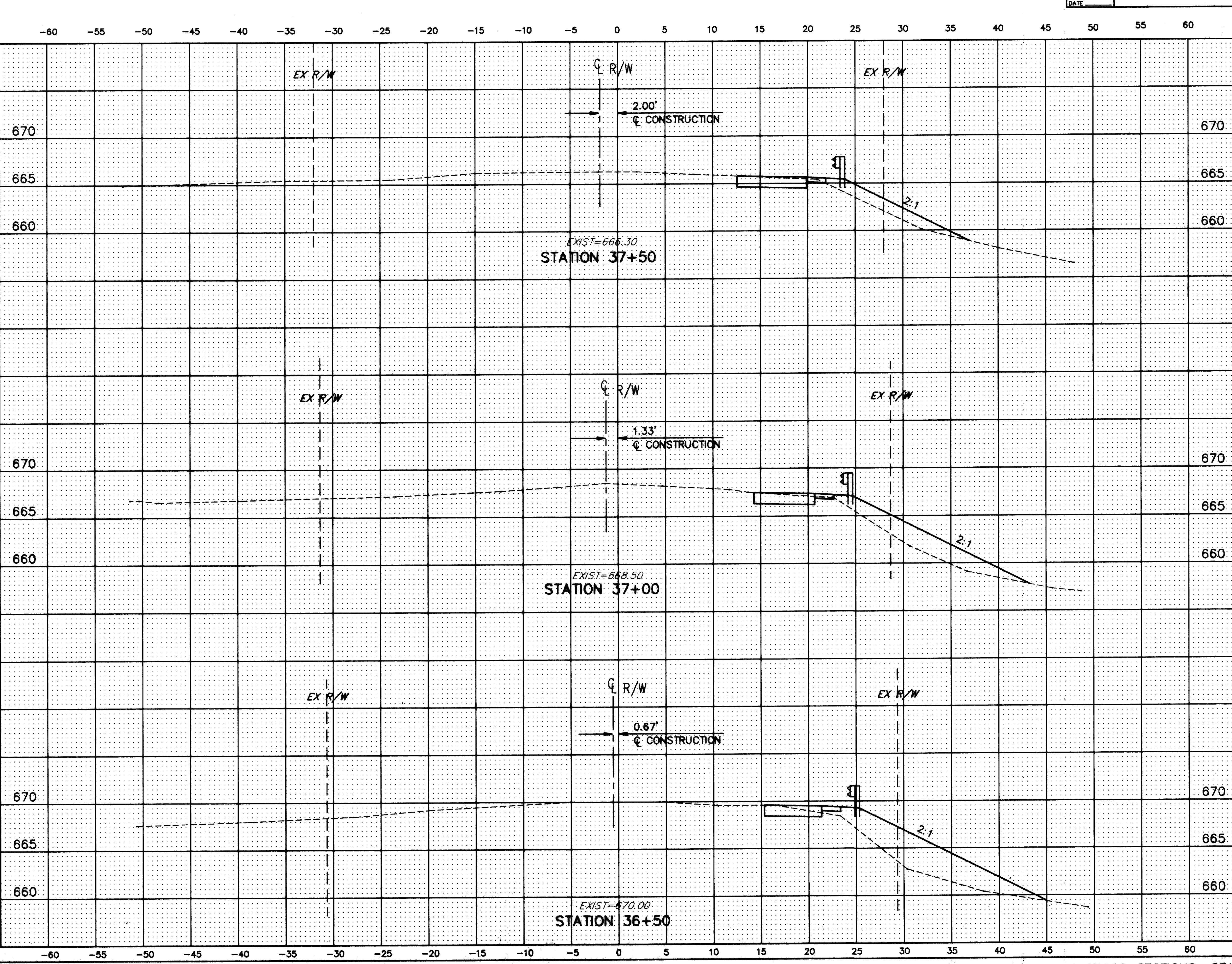
HOPKINS ROAD CROSS-SECTIONS STA. 36+50 TO STA. 37+50
