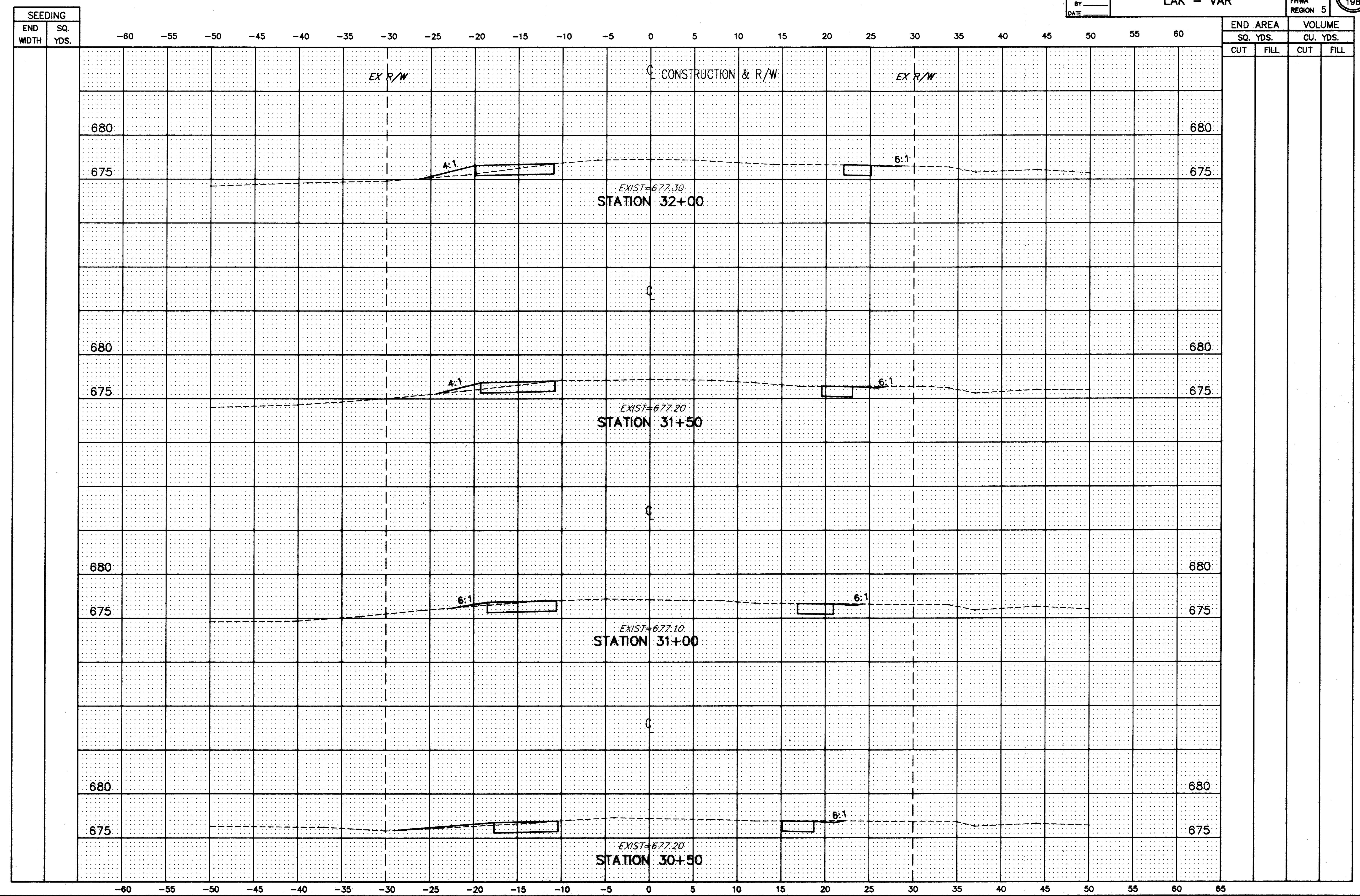
HOPKINS ROAD CROSS-SECTIONS STA. 30+50 TO STA. 32+00
