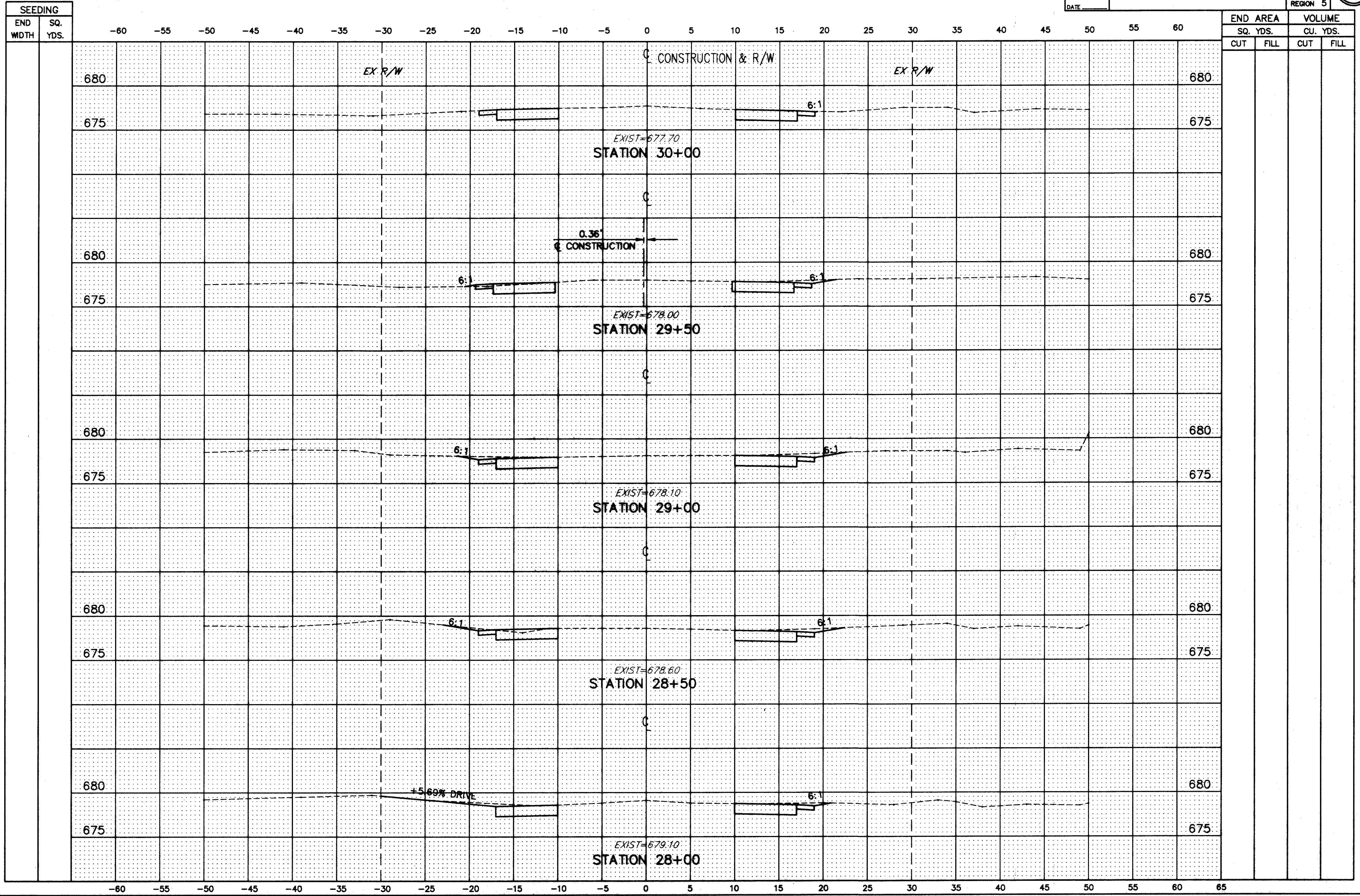
HOPKINS ROAD CROSS-SECTIONS STA. 28+00 TO STA. 30+00
