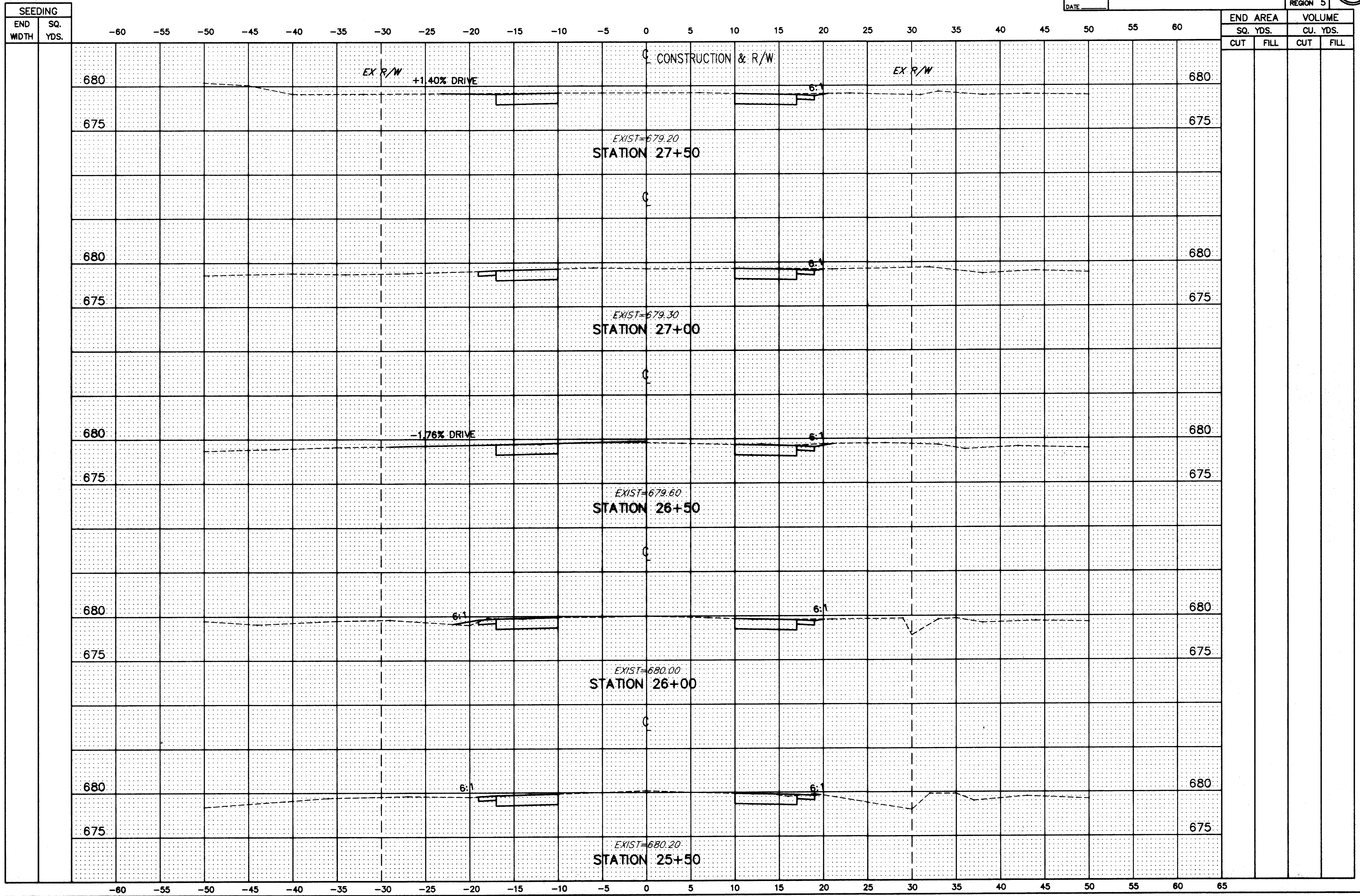
HOPKINS ROAD CROSS-SECTIONS STA. 25+50 TO STA. 27+50
