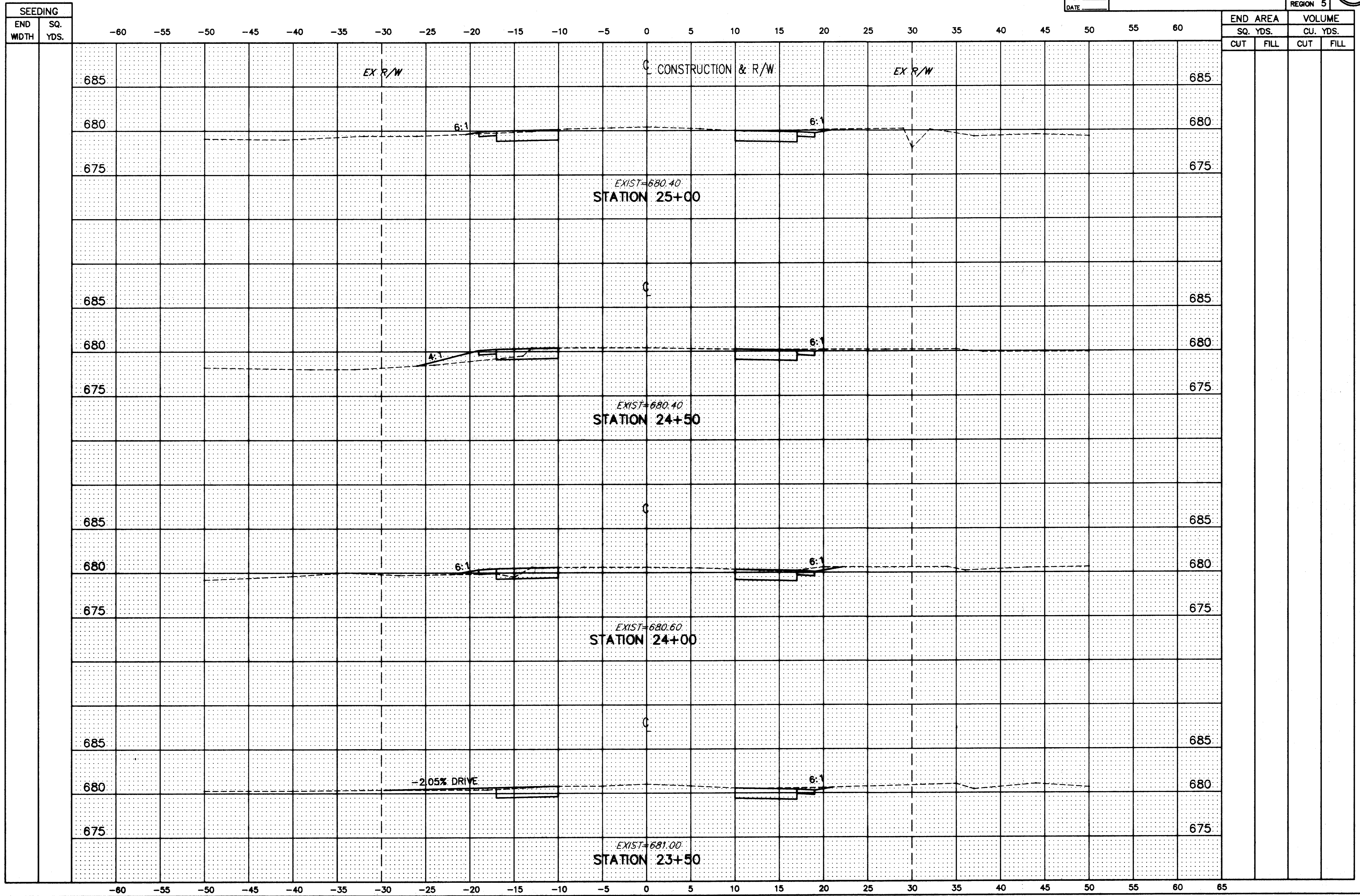
HOPKINS ROAD CROSS-SECTIONS STA. 23+50 TO STA. 25+00
