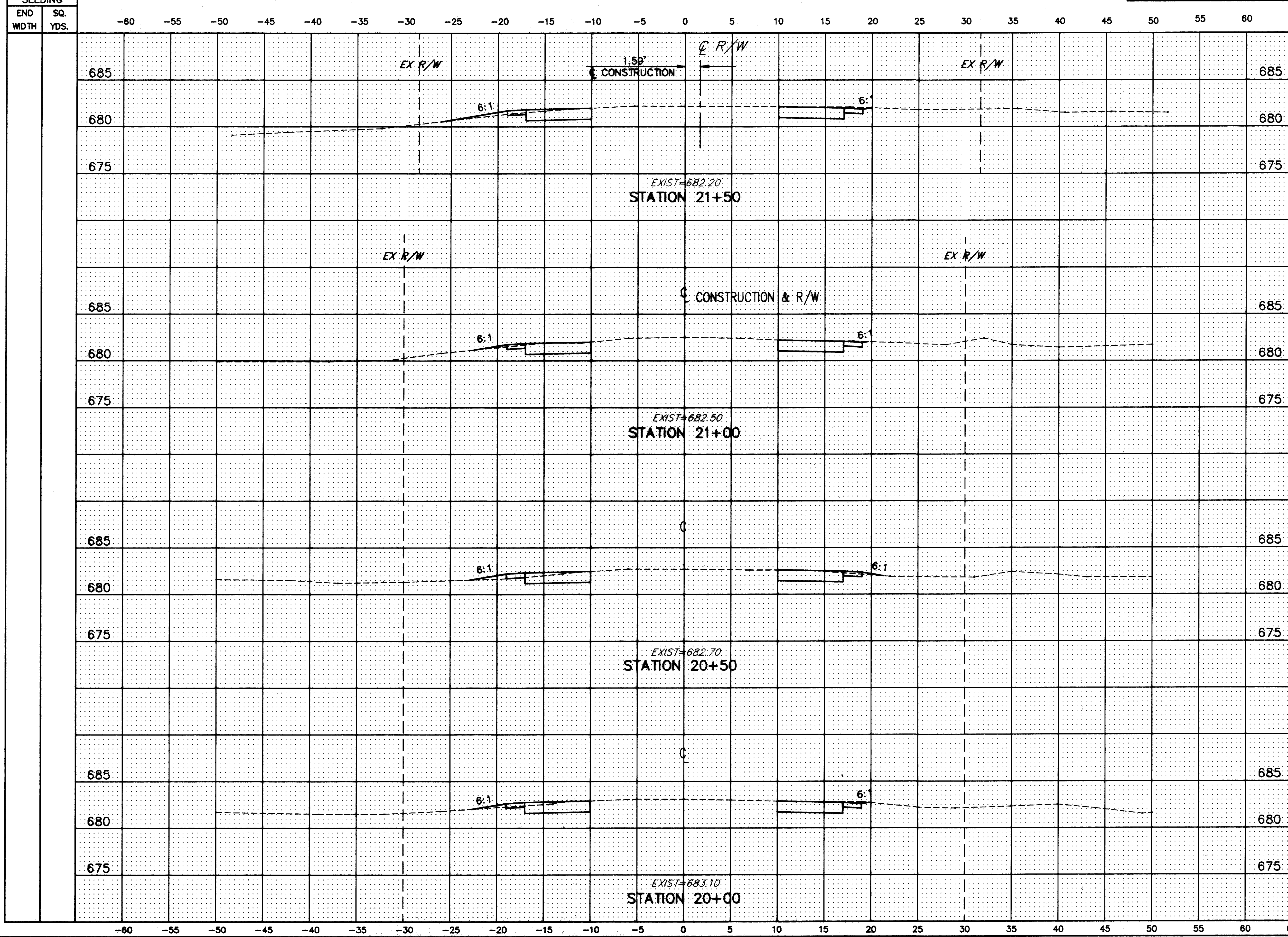
HOPKINS ROAD CROSS-SECTIONS STA. 20+00 TO STA. 21+50
