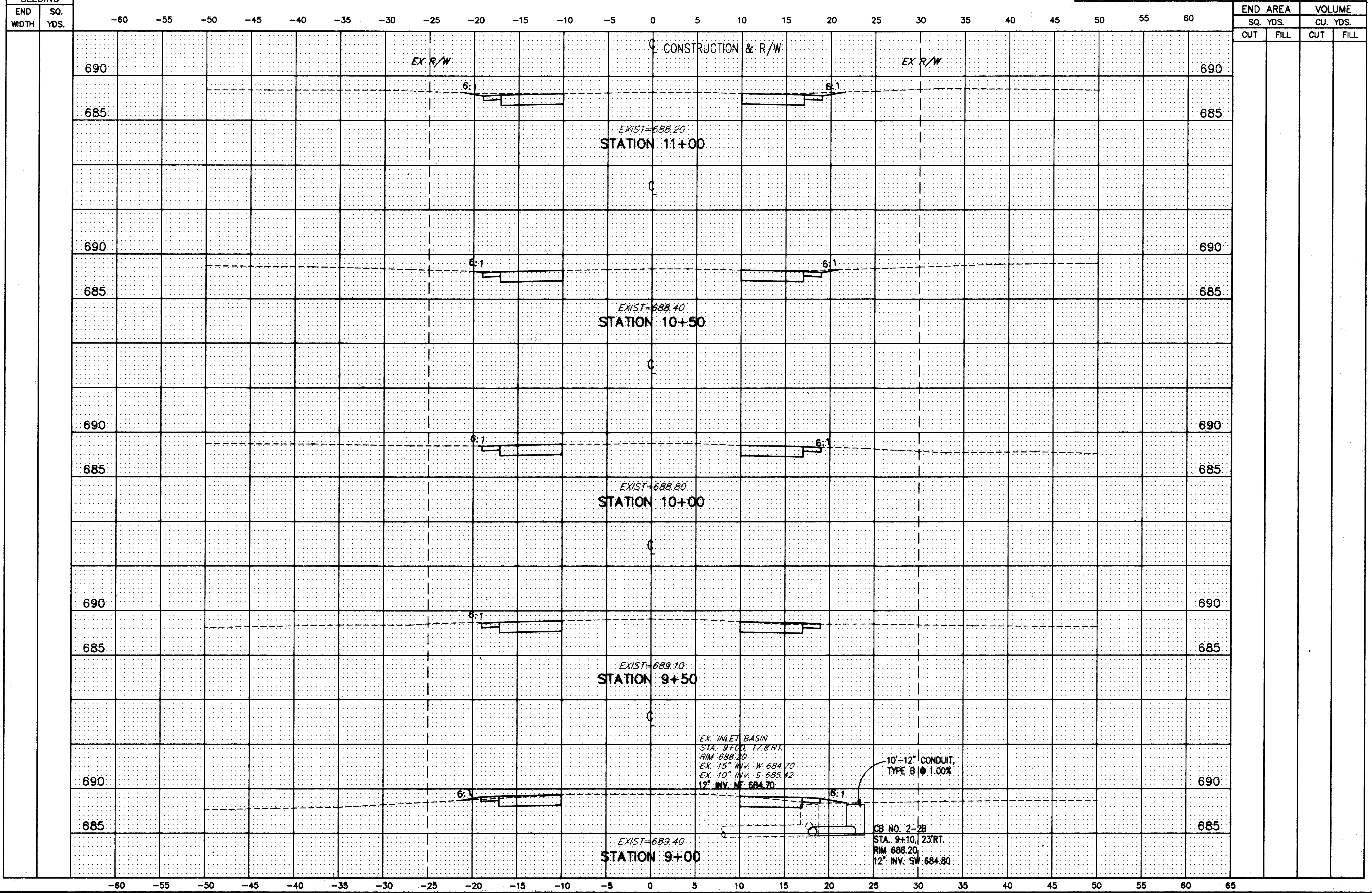
HOPKINS ROAD CROSS-SECTIONS STA. 9+00 TO STA. 11+00
