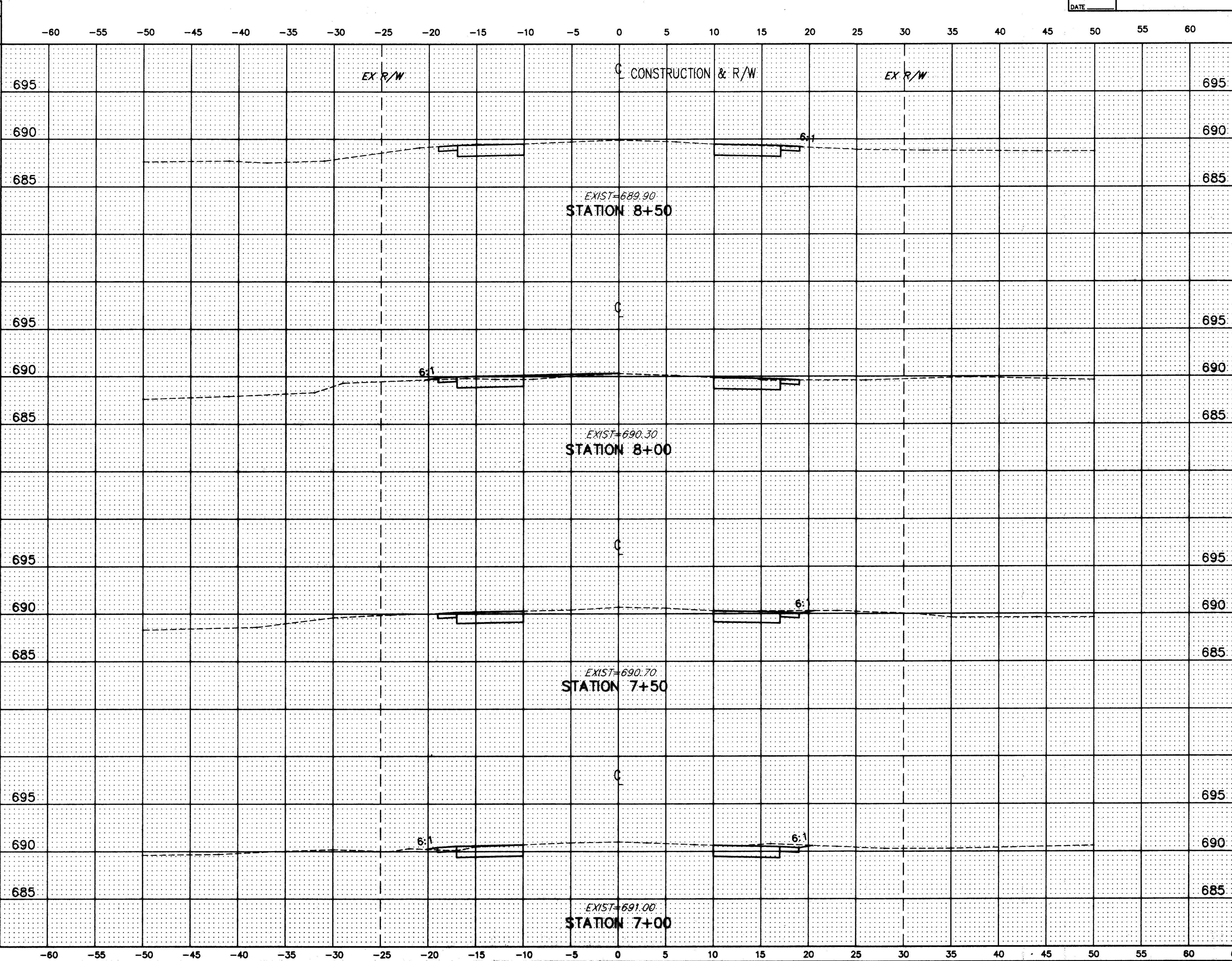
HOPKINS ROAD CROSS-SECTIONS STA. 7+00 TO STA. 8+50
