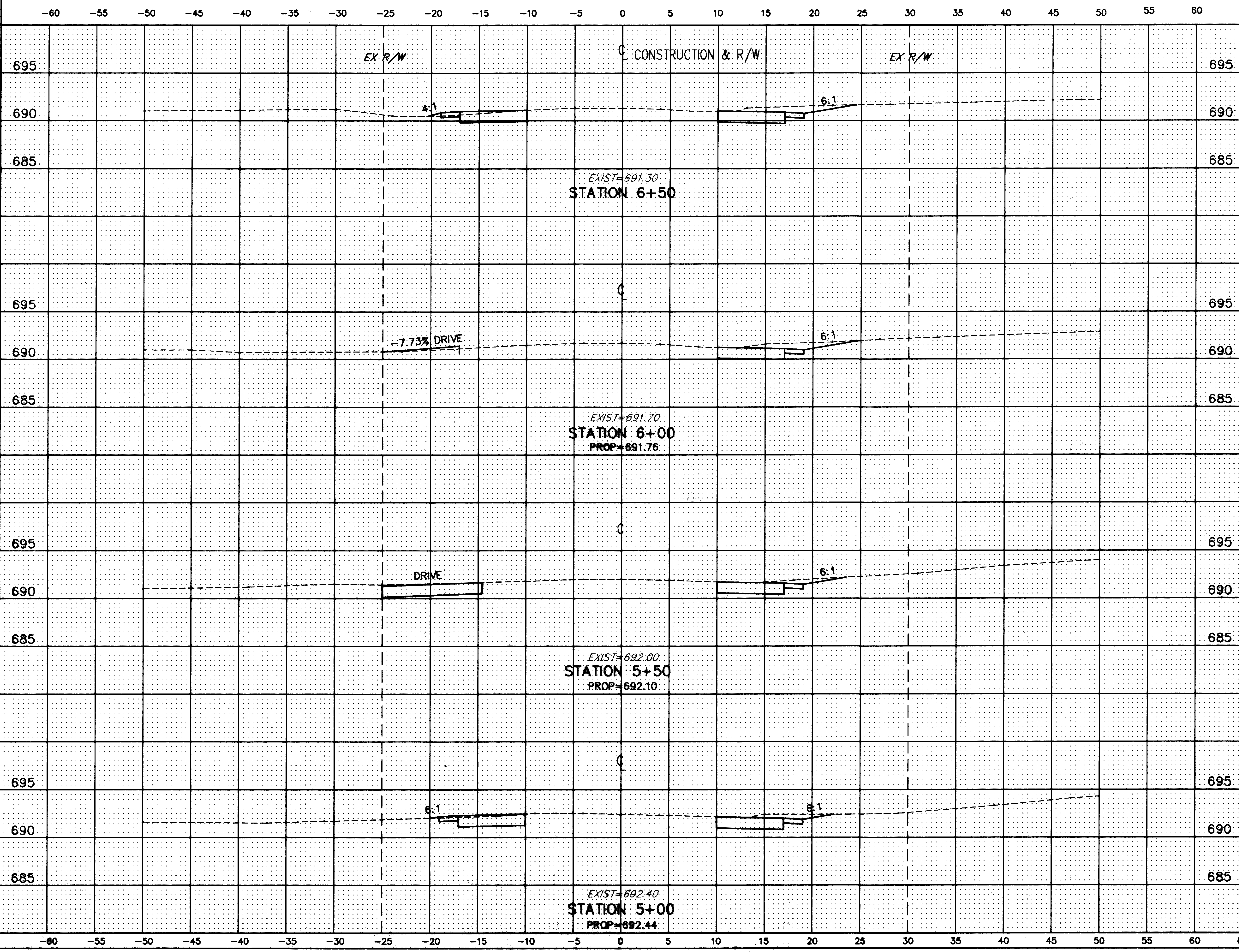
HOPKINS ROAD CROSS-SECTIONS STA. 5+00 TO STA. 6+50
