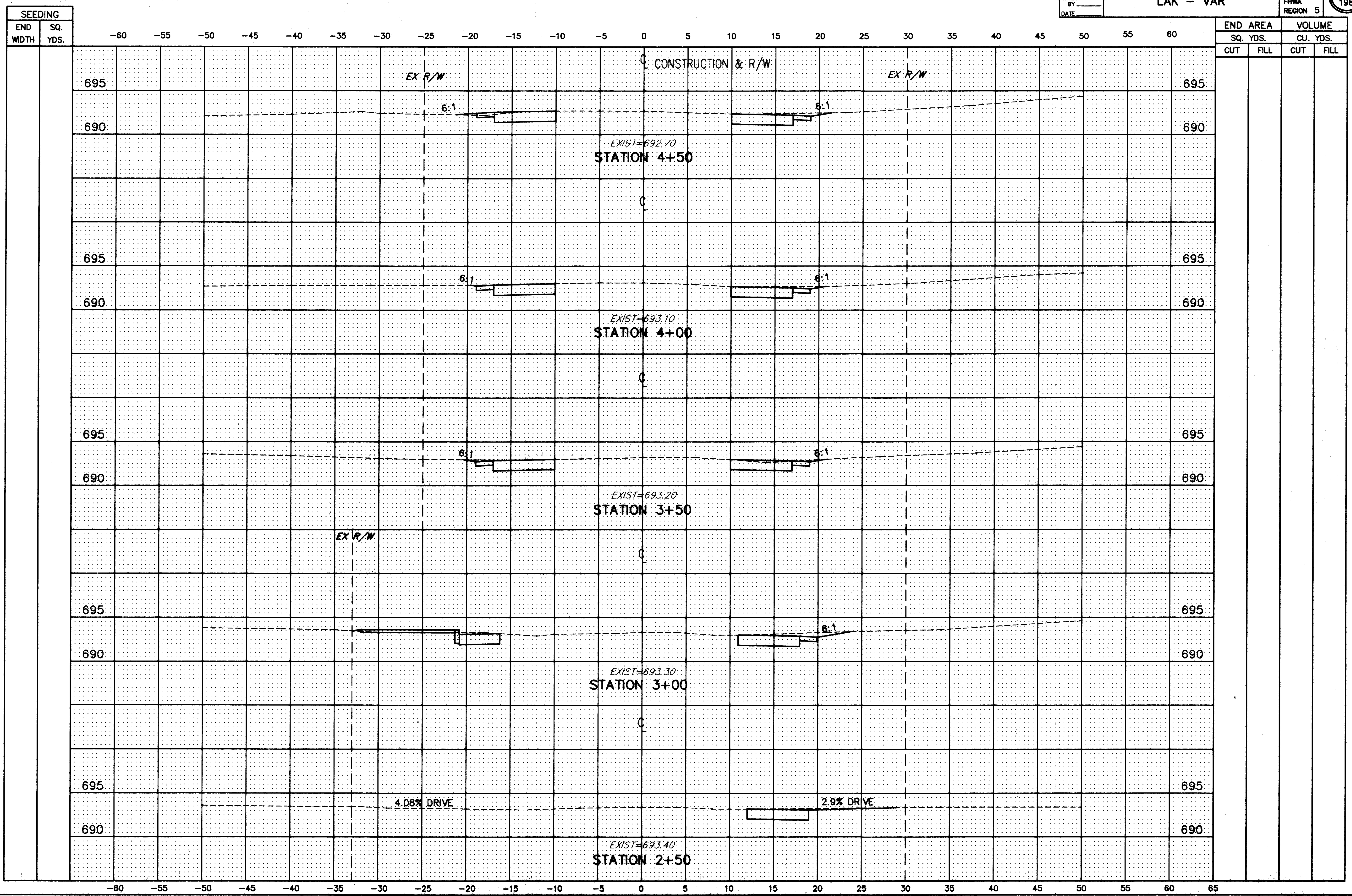
HOPKINS ROAD CROSS-SECTIONS STA. 2+50 TO STA. 4+50
