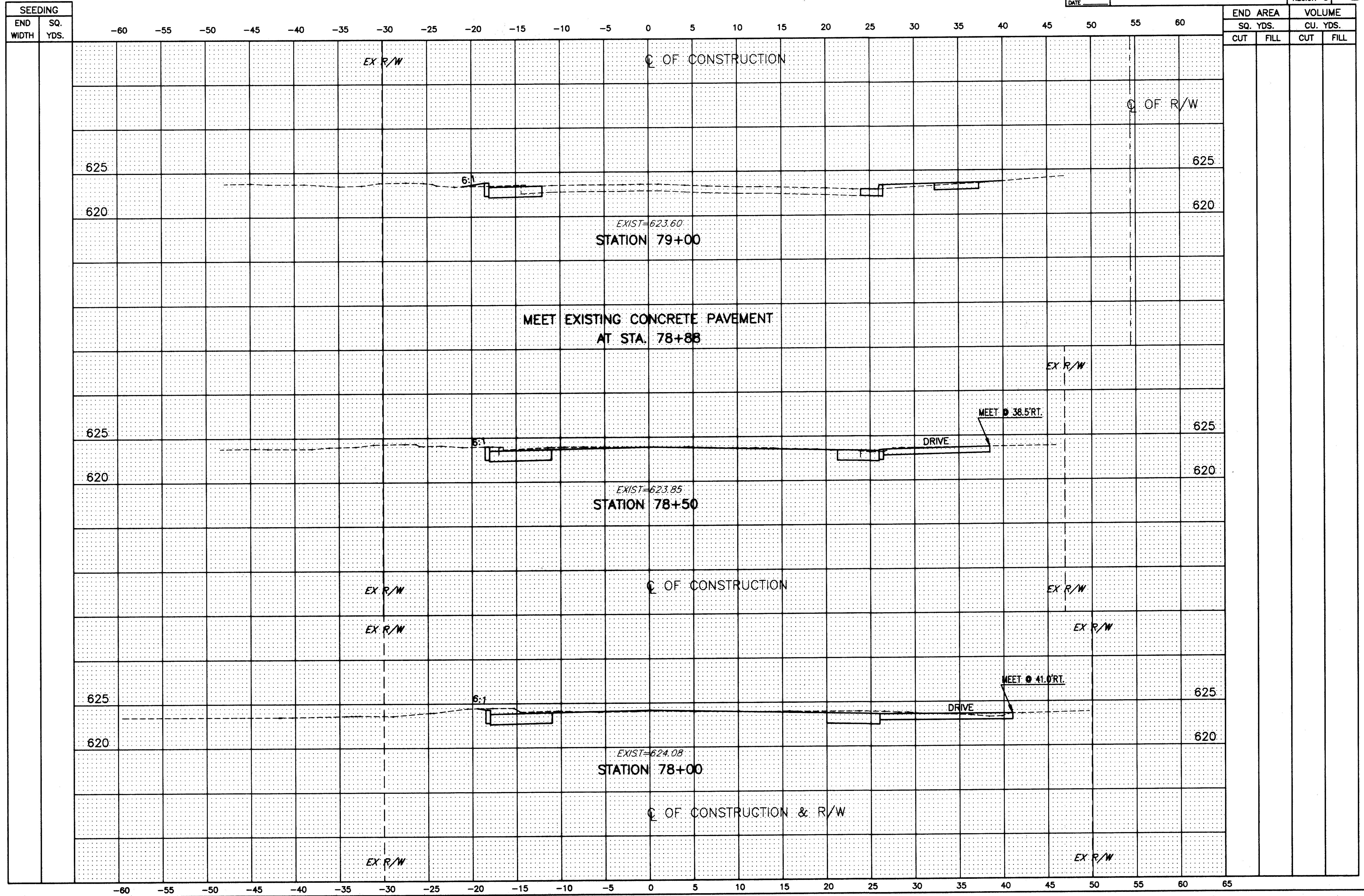
MUNSON ROAD CROSS-SECTIONS STA. 78+00 TO STA. 79+00
