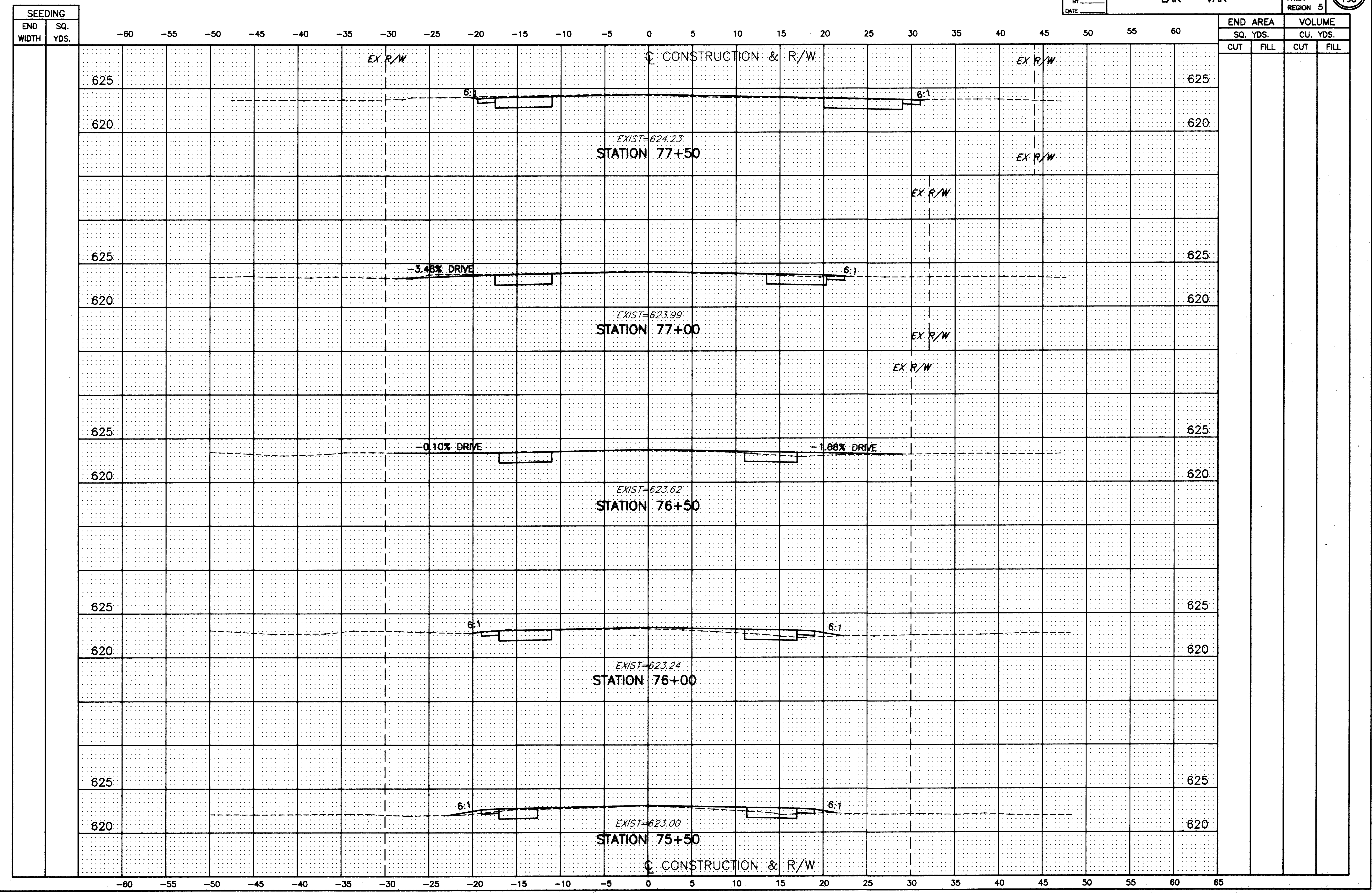
MUNSON ROAD CROSS-SECTIONS STA. 75+50 TO STA. 77+50
