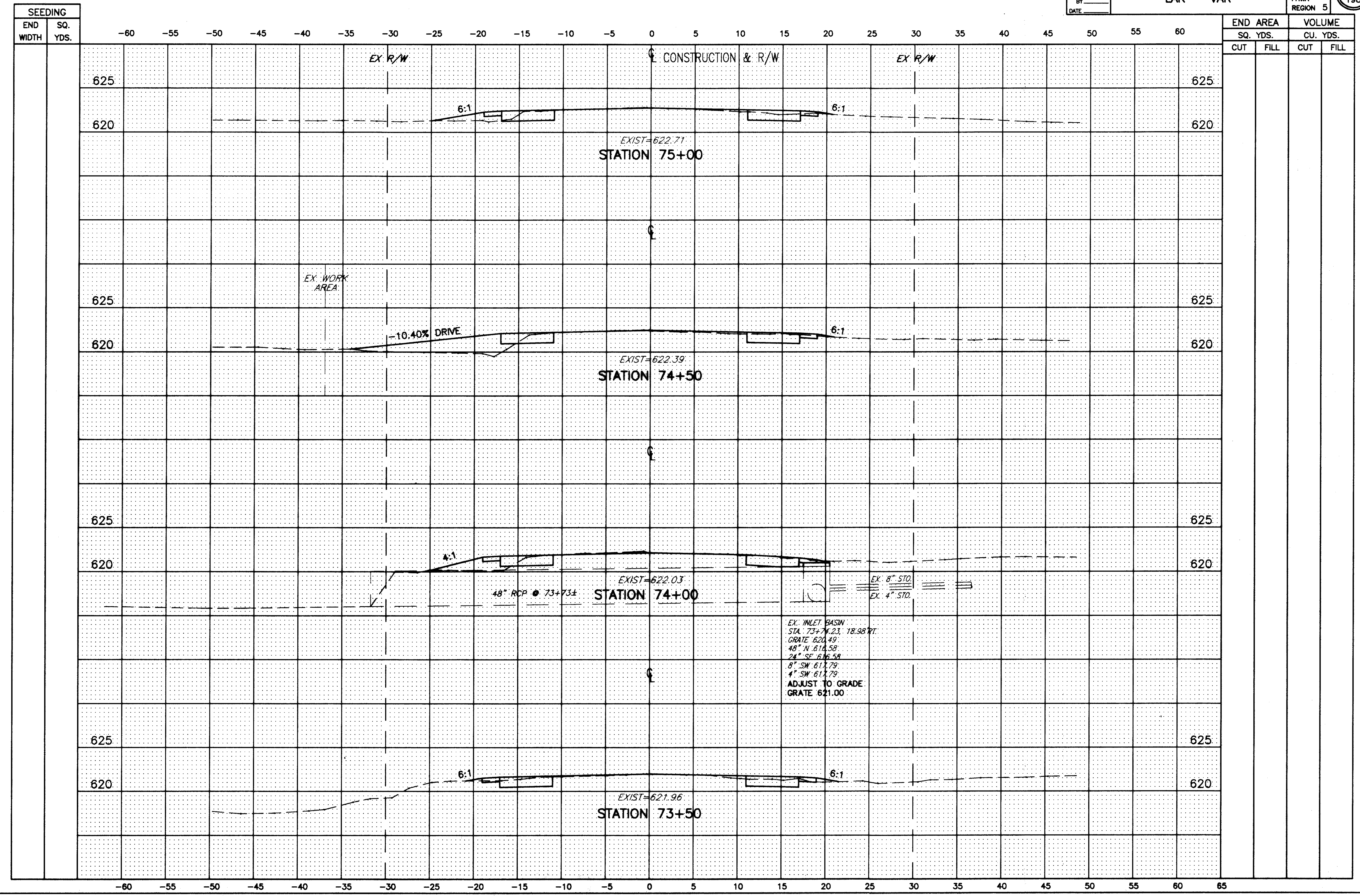
MUNSON ROAD CROSS-SECTIONS STA. 73+50 TO STA. 75+00
