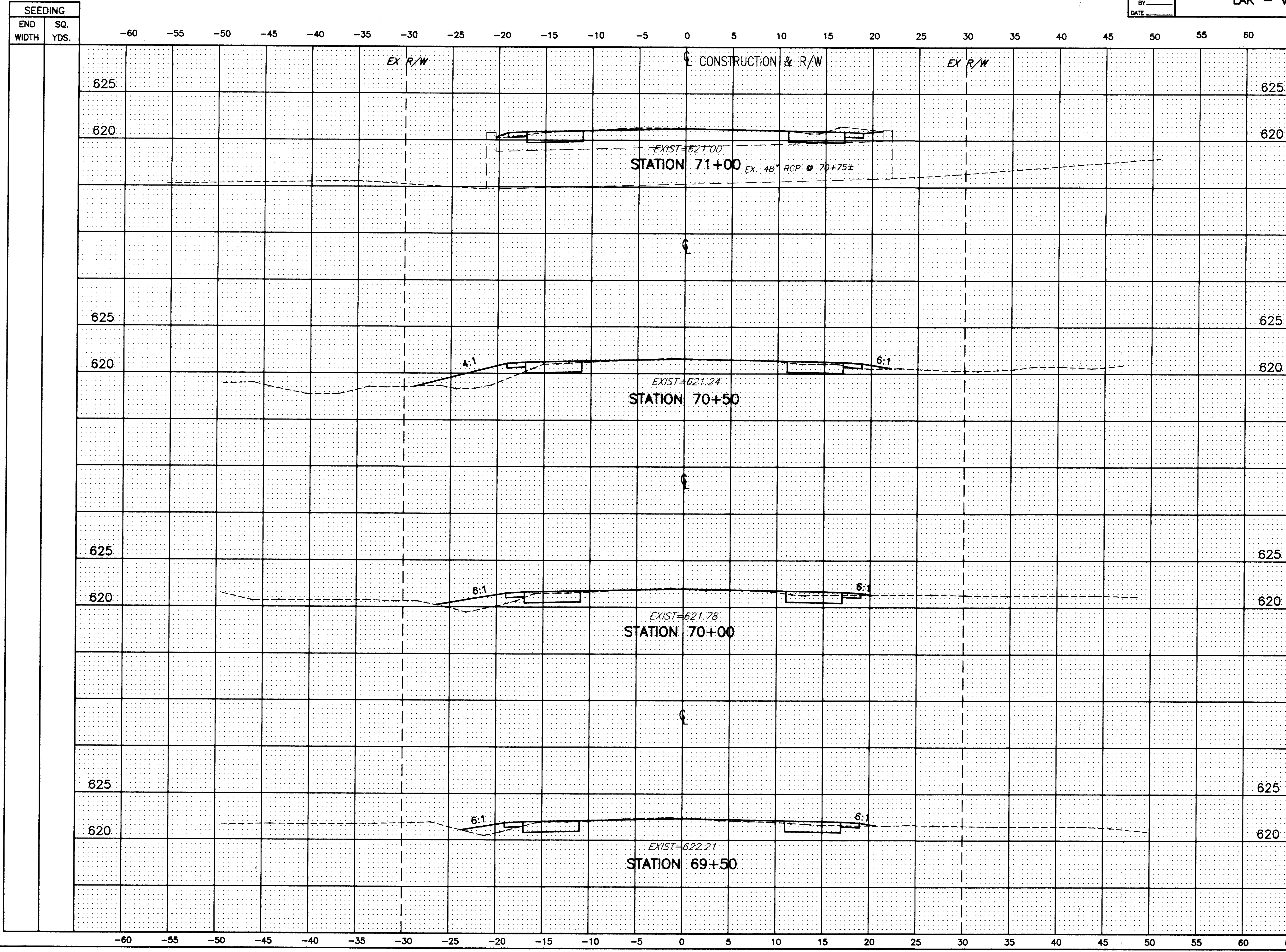
MUNSON ROAD CROSS-SECTIONS STA. 69+50 TO STA. 71+00
