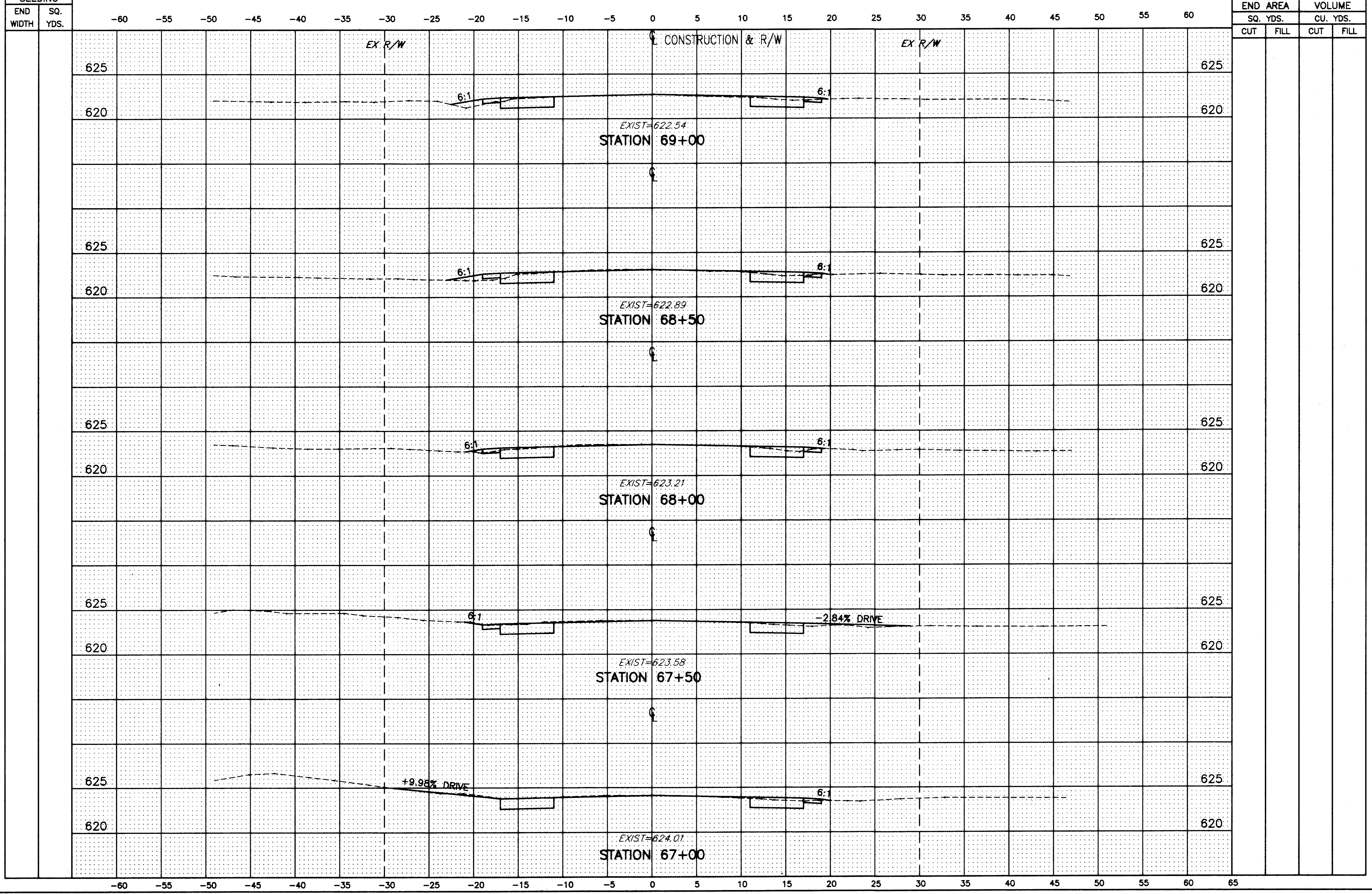
MUNSON ROAD CROSS-SECTIONS STA. 67+00 TO STA. 69+00
