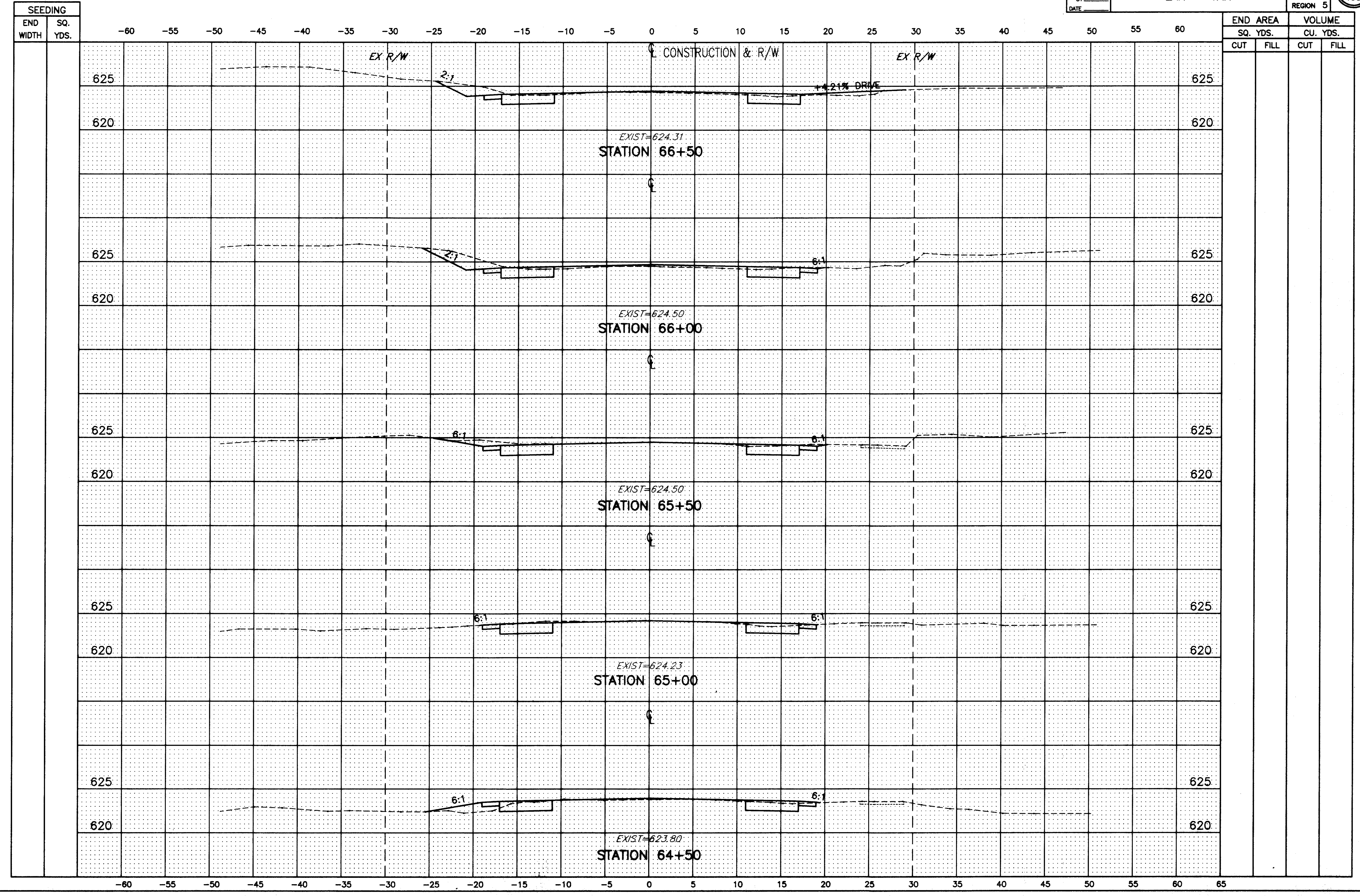
MUNSON ROAD CROSS-SECTIONS STA. 64+50 TO STA. 66+50
