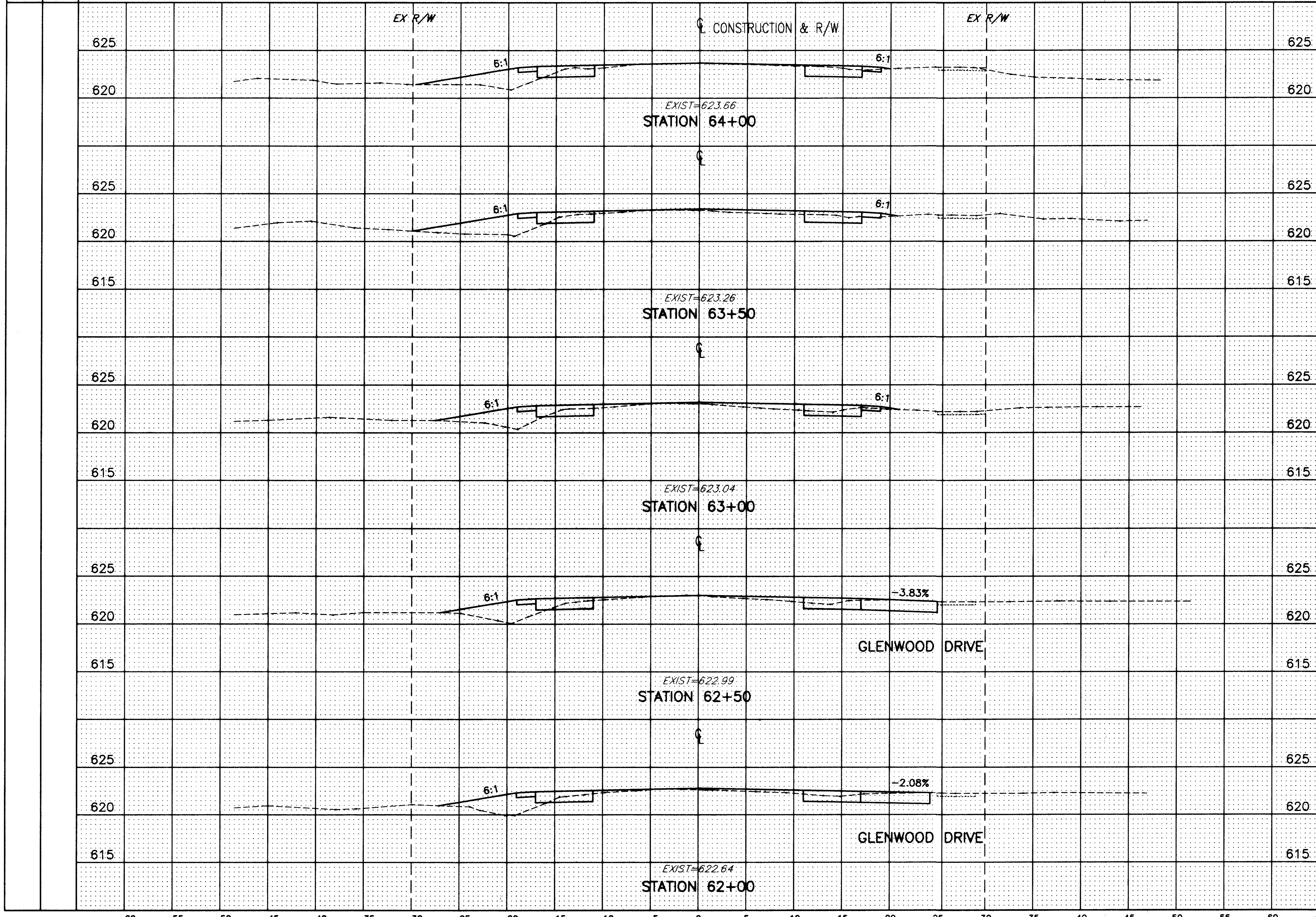
MUNSON ROAD CROSS-SECTIONS STA. 62+00 TO STA. 64+00
