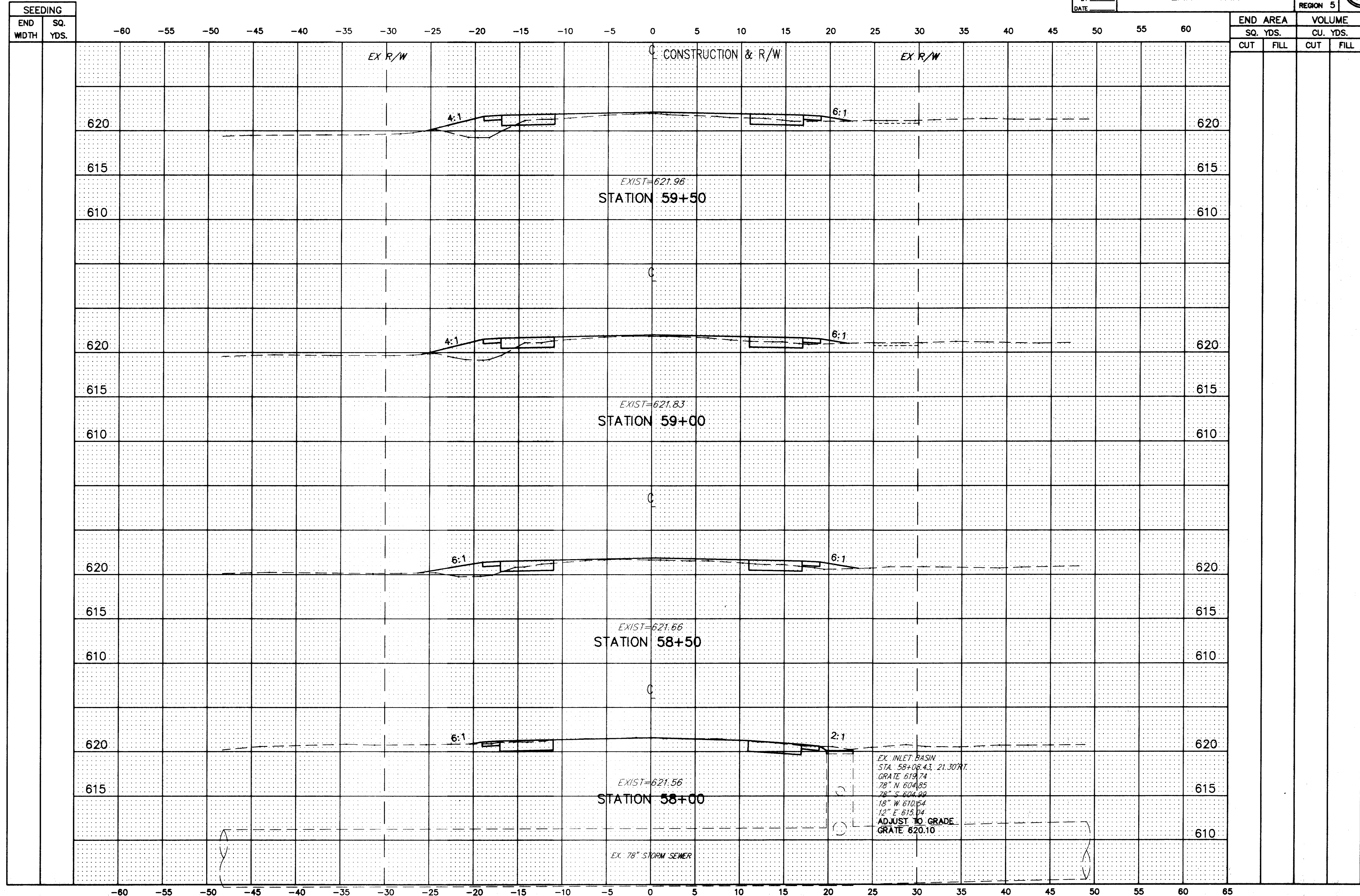
MUNSON ROAD CROSS-SECTIONS STA. 58+00 TO STA. 59+50
