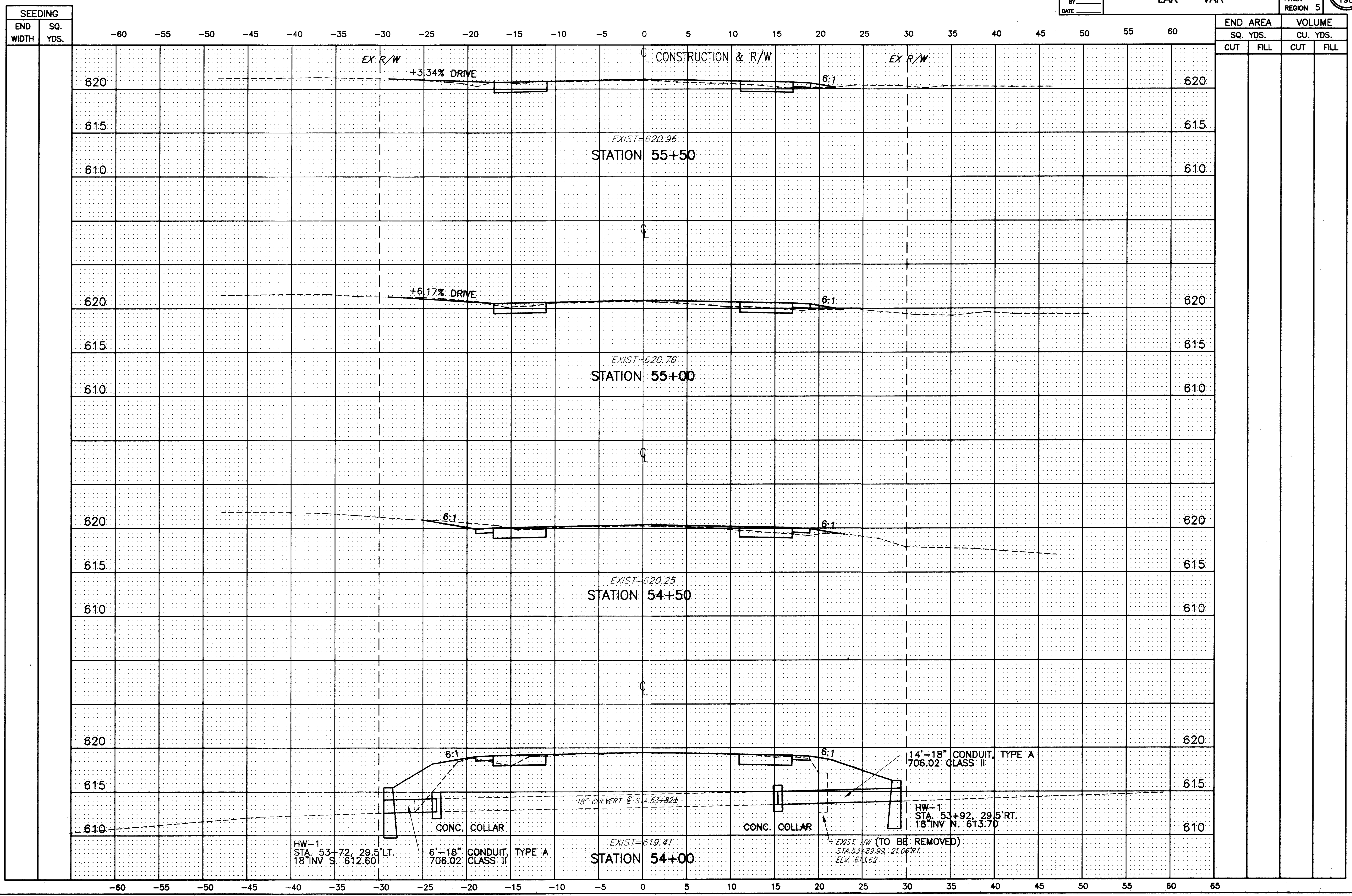
MUNSON ROAD CROSS-SECTIONS STA. 54+00 TO STA. 55+50
