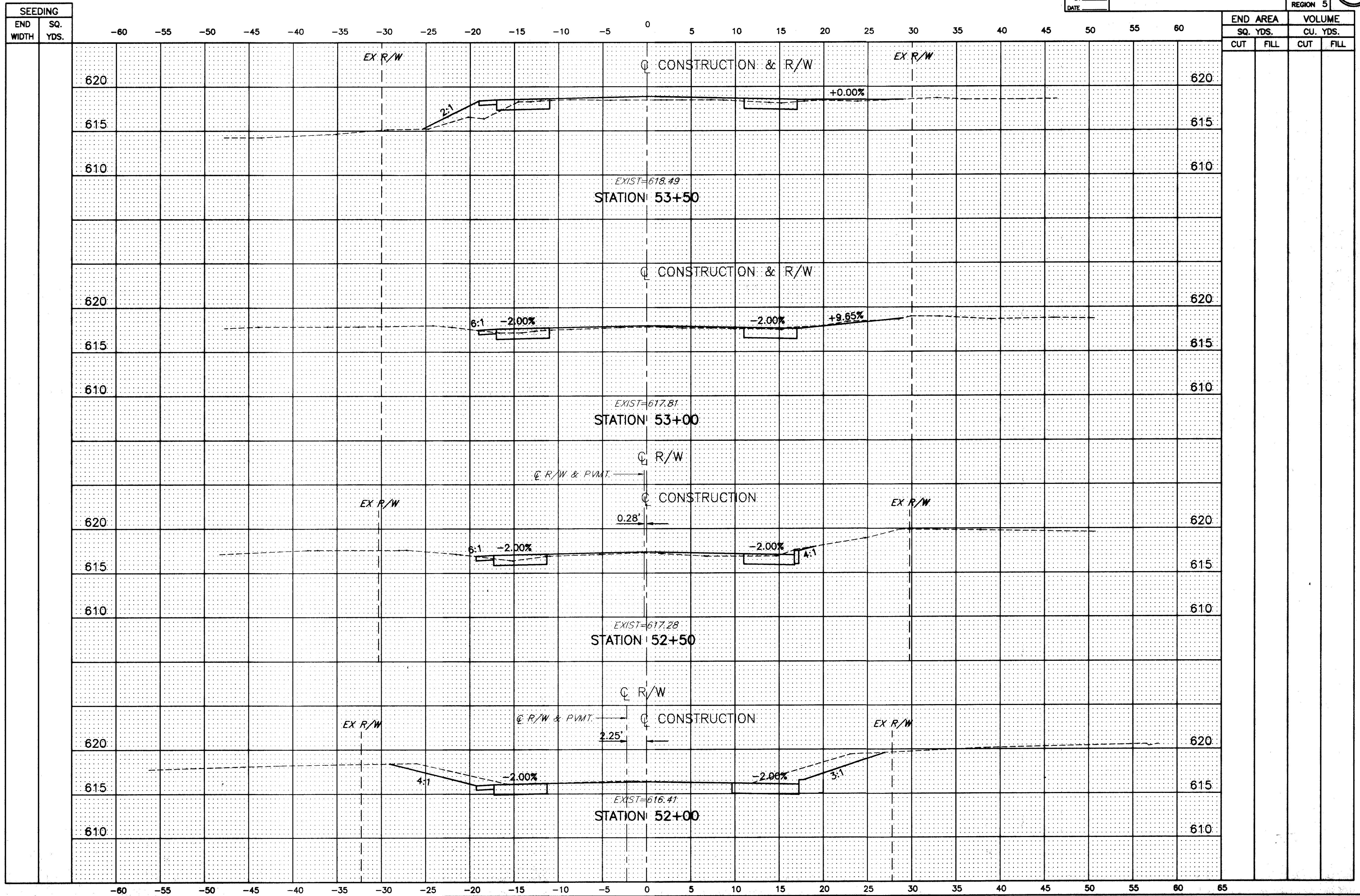
MUNSON ROAD CROSS-SECTIONS STA. 52+00 TO STA. 53+50
