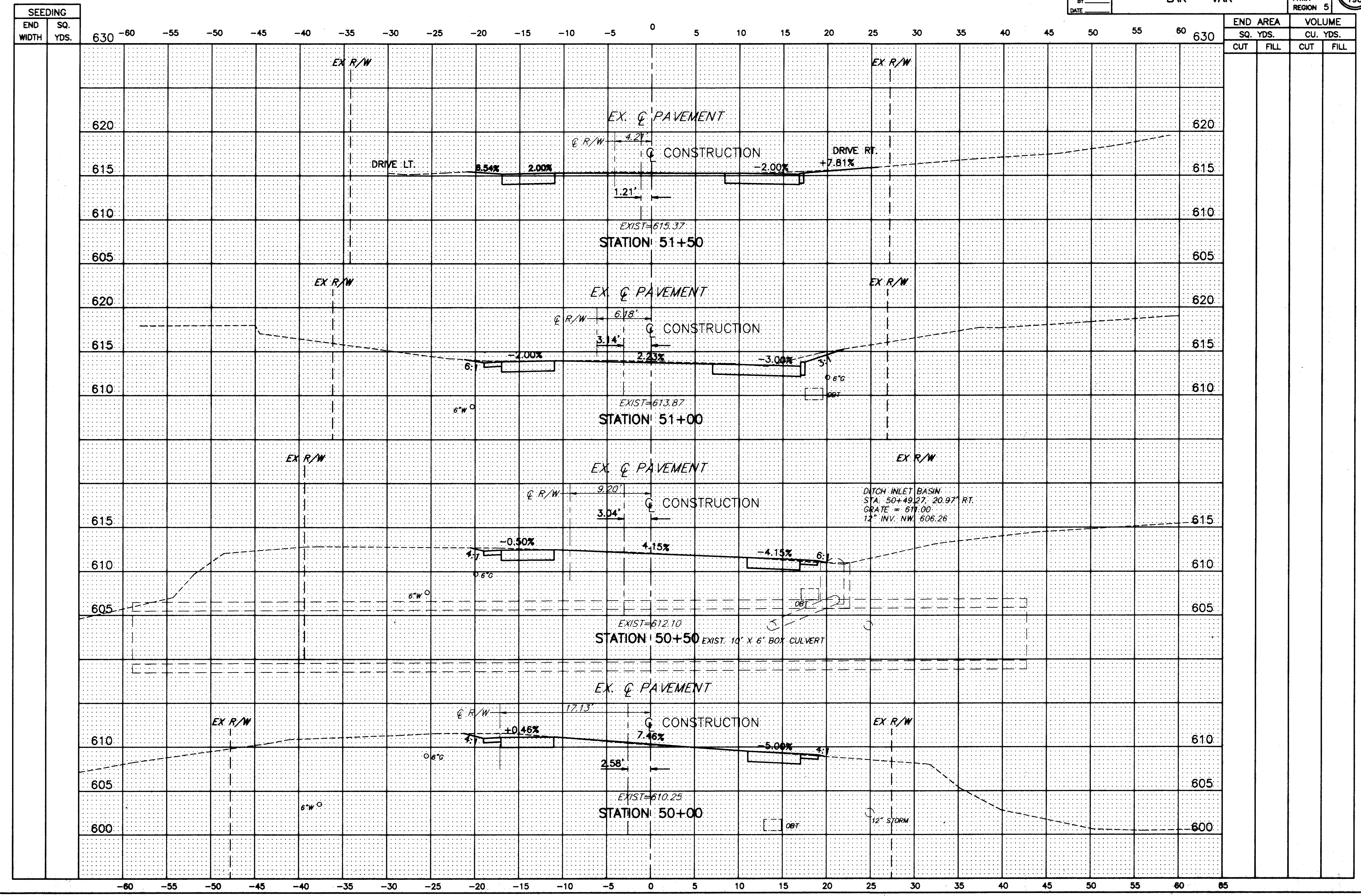
MUNSON ROAD CROSS-SECTIONS STA. 50+00 TO STA. 51+50
