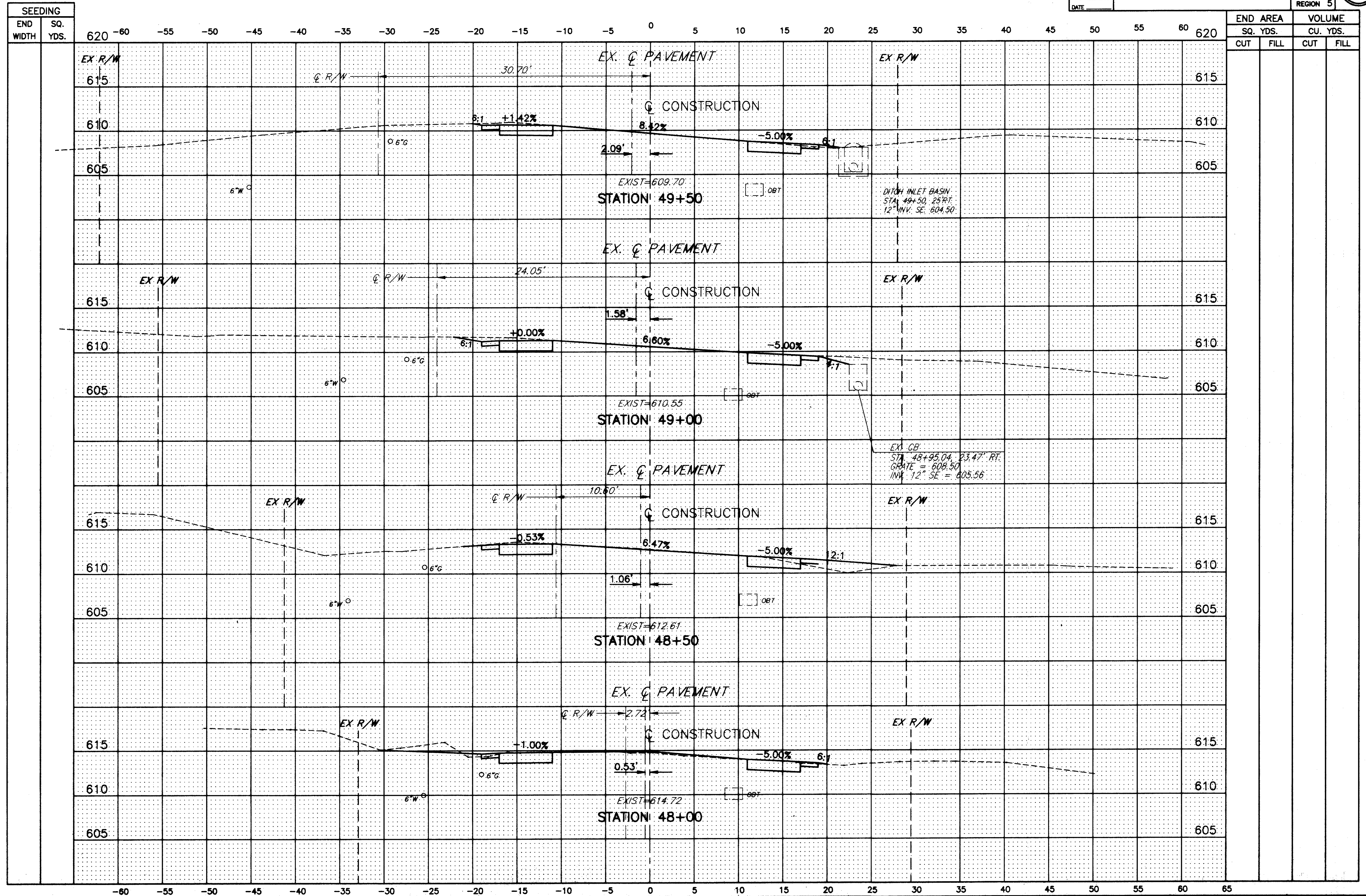
MUNSON ROAD CROSS-SECTIONS STA. 48+00 TO STA. 49+50
