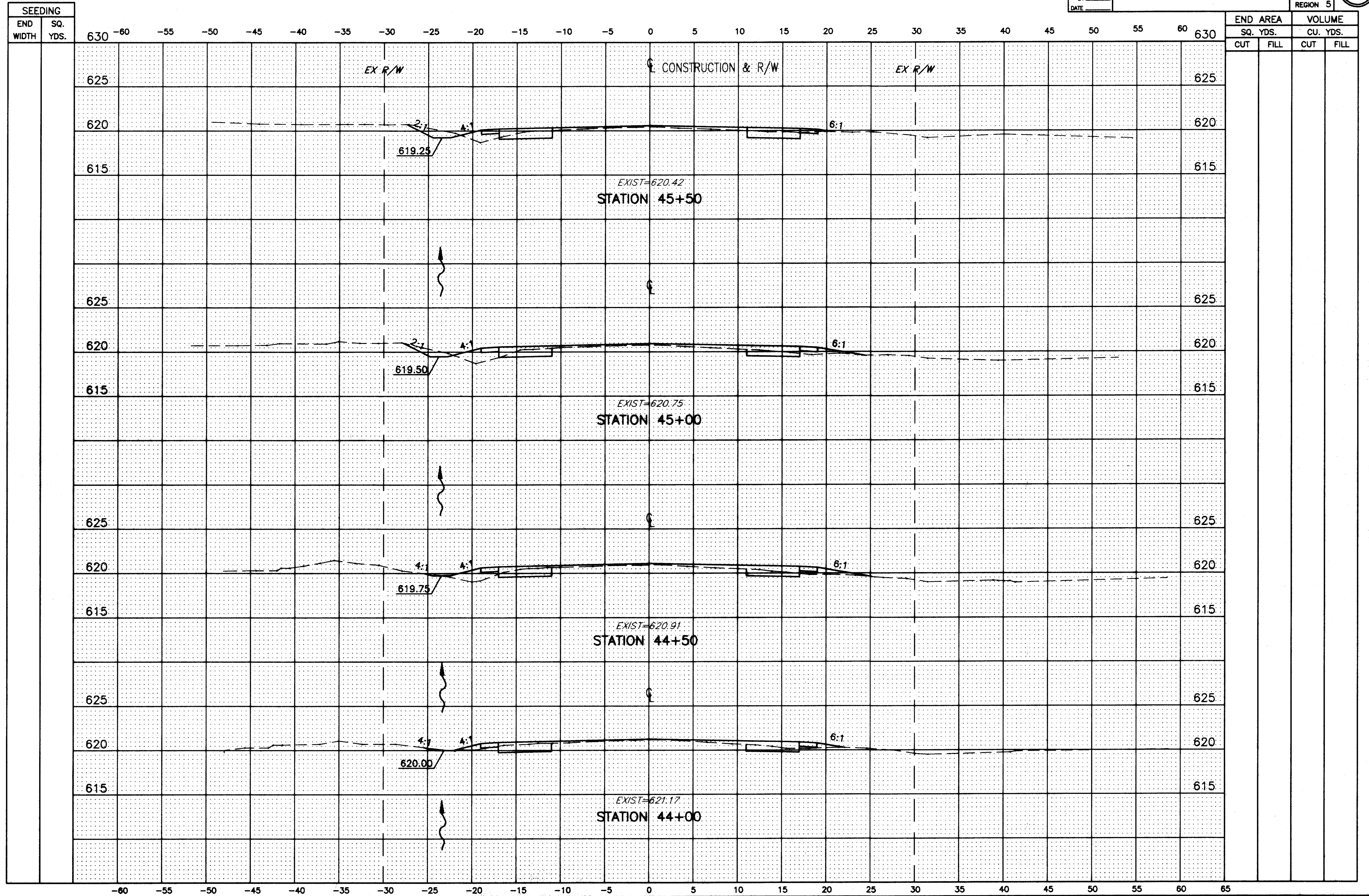
MUNSON ROAD CROSS-SECTIONS STA. 44+00 TO STA. 45+50
