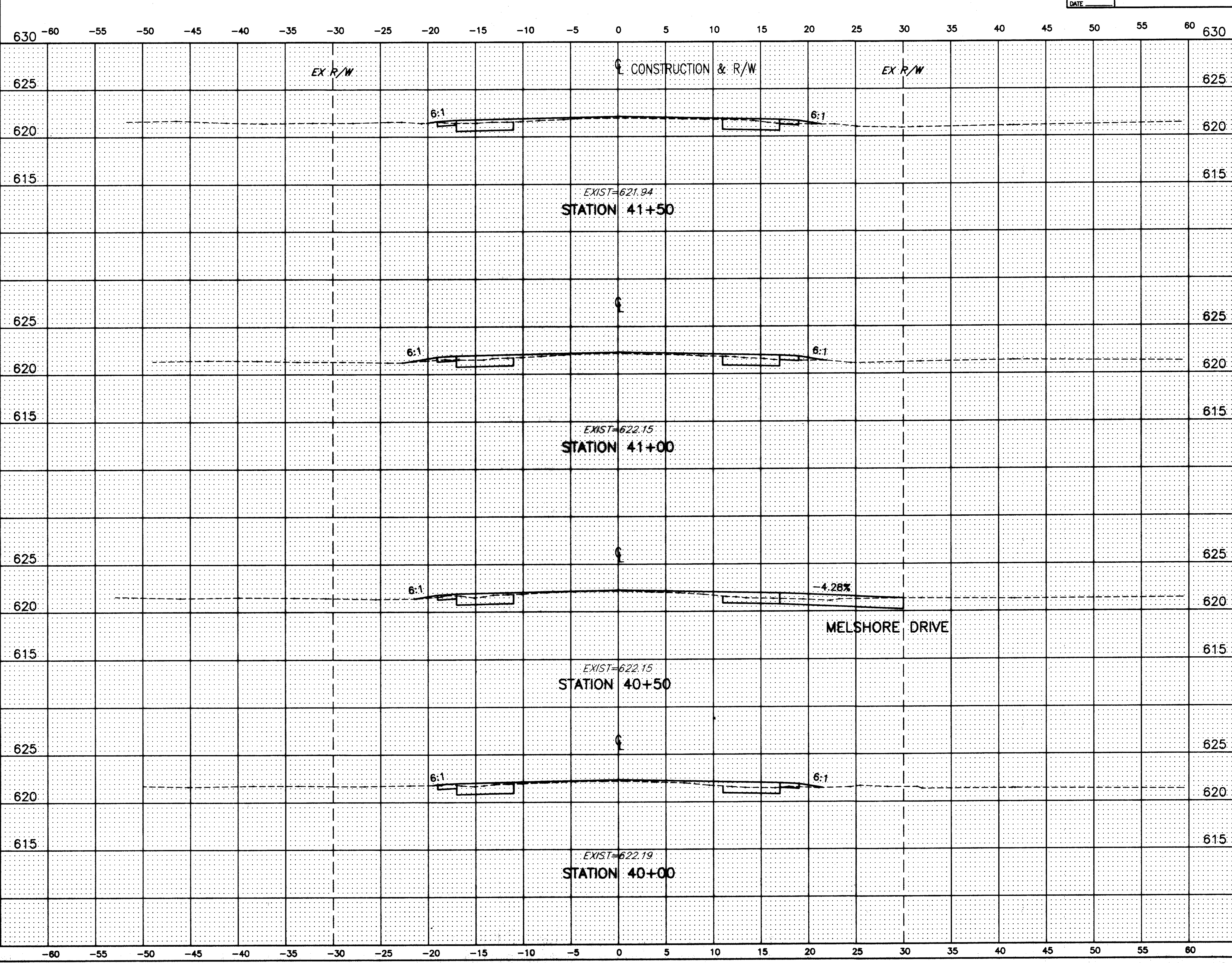
MUNSON ROAD CROSS-SECTIONS STA. 40+00 TO STA. 41+50
