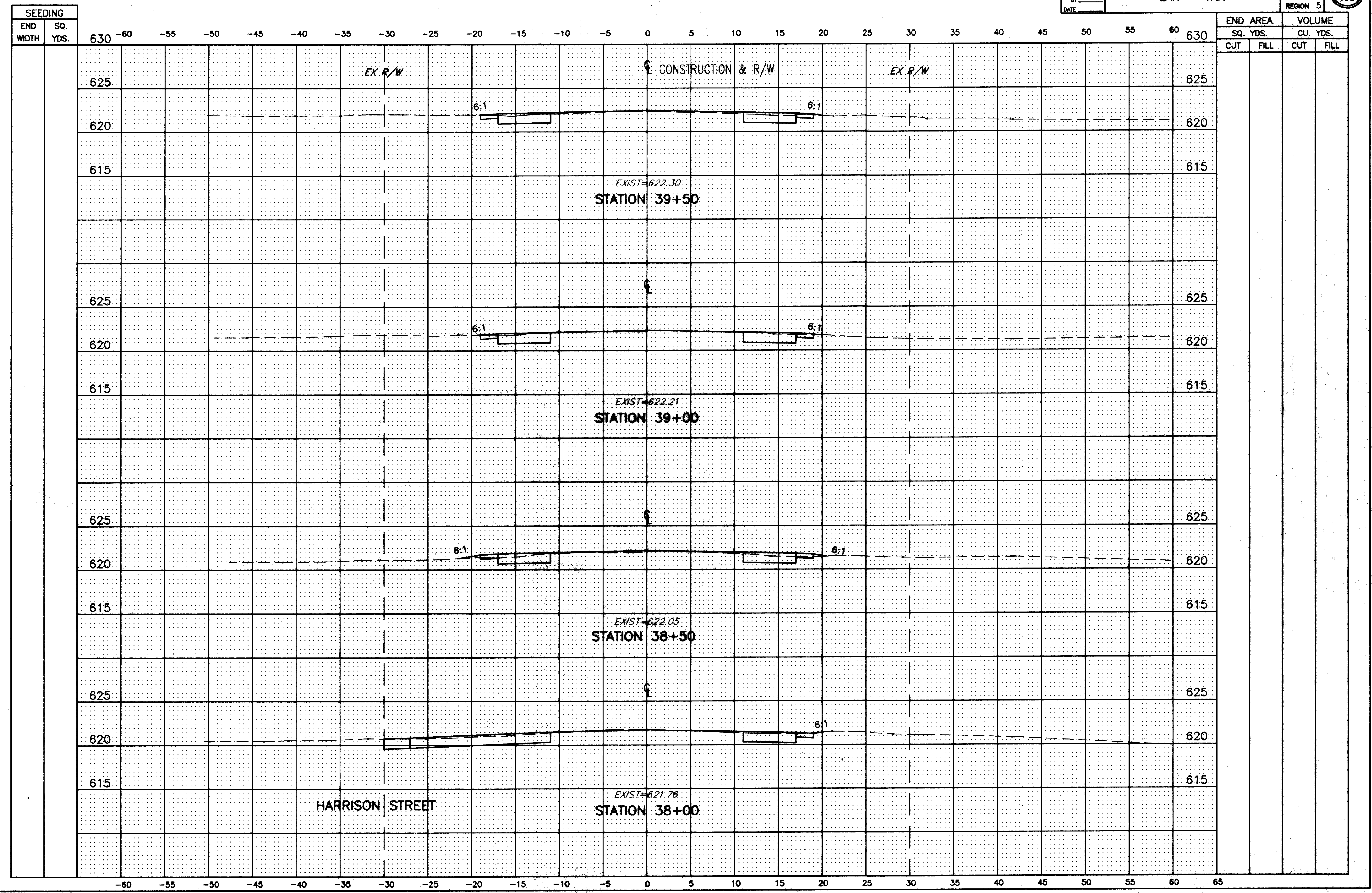
MUNSON ROAD CROSS-SECTIONS STA. 38+00 TO STA. 39+50
