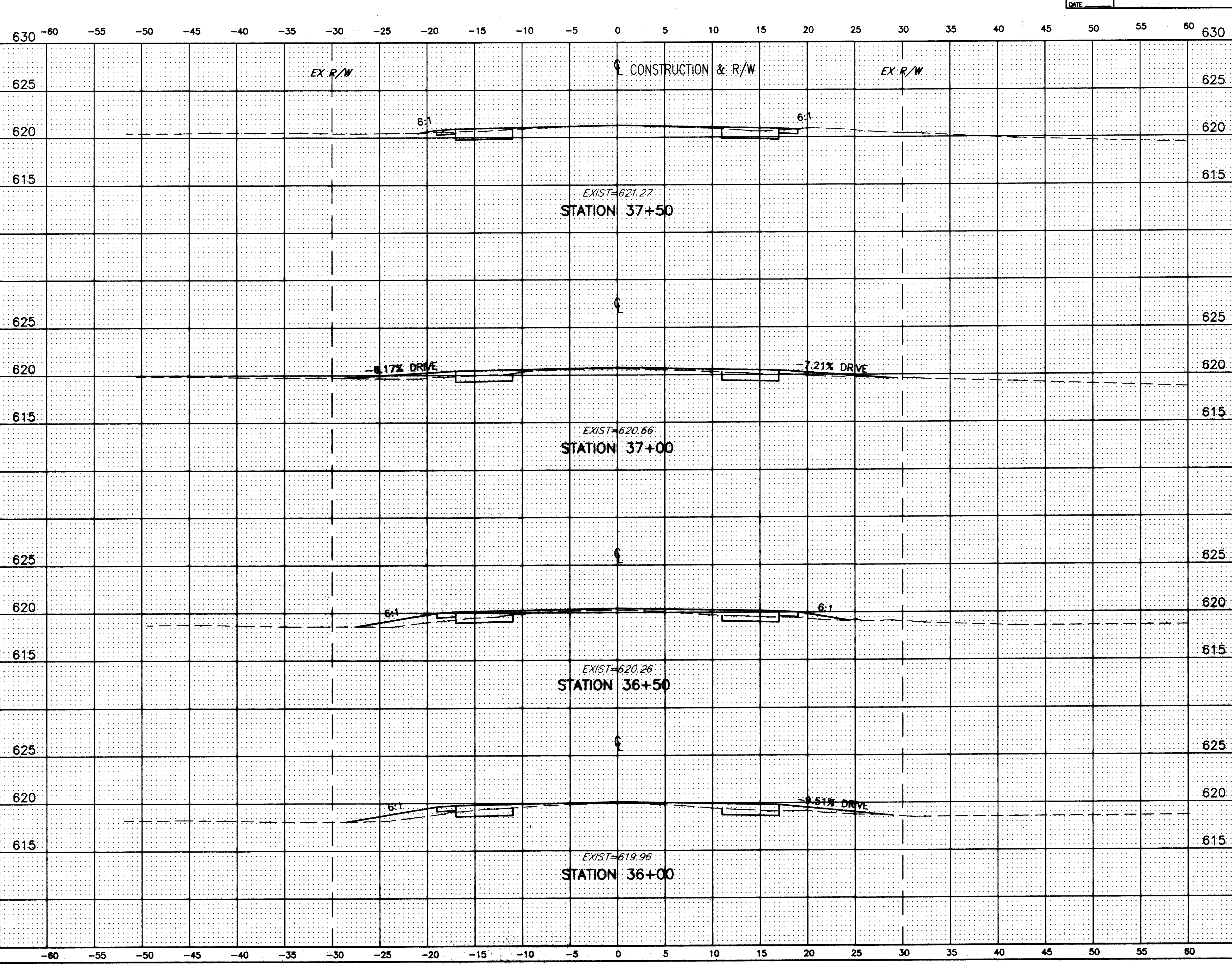
MUNSON ROAD CROSS-SECTIONS STA. 36+00 TO STA. 37+50
