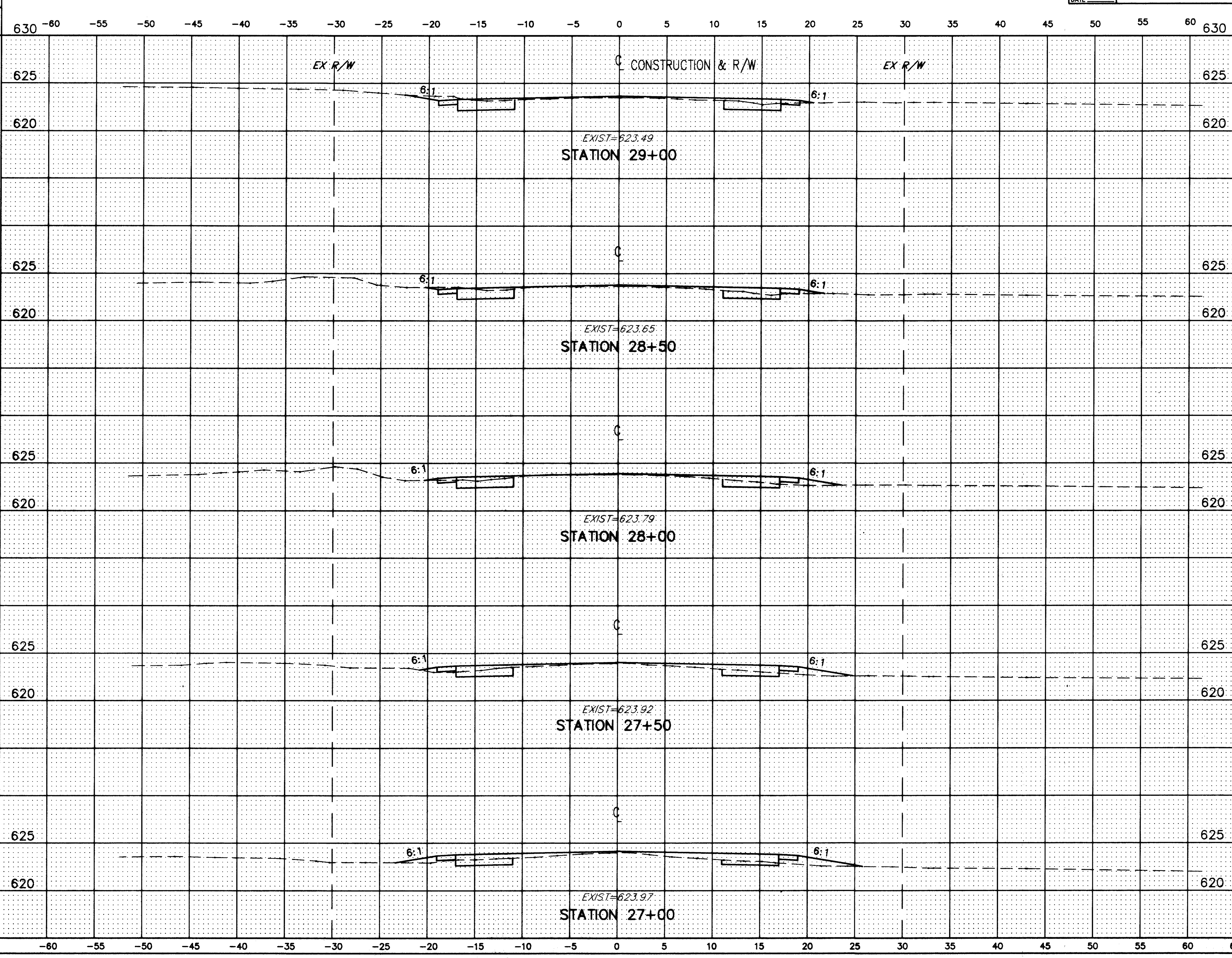
MUNSON ROAD CROSS-SECTIONS STA. 27+00 TO STA. 29+00
