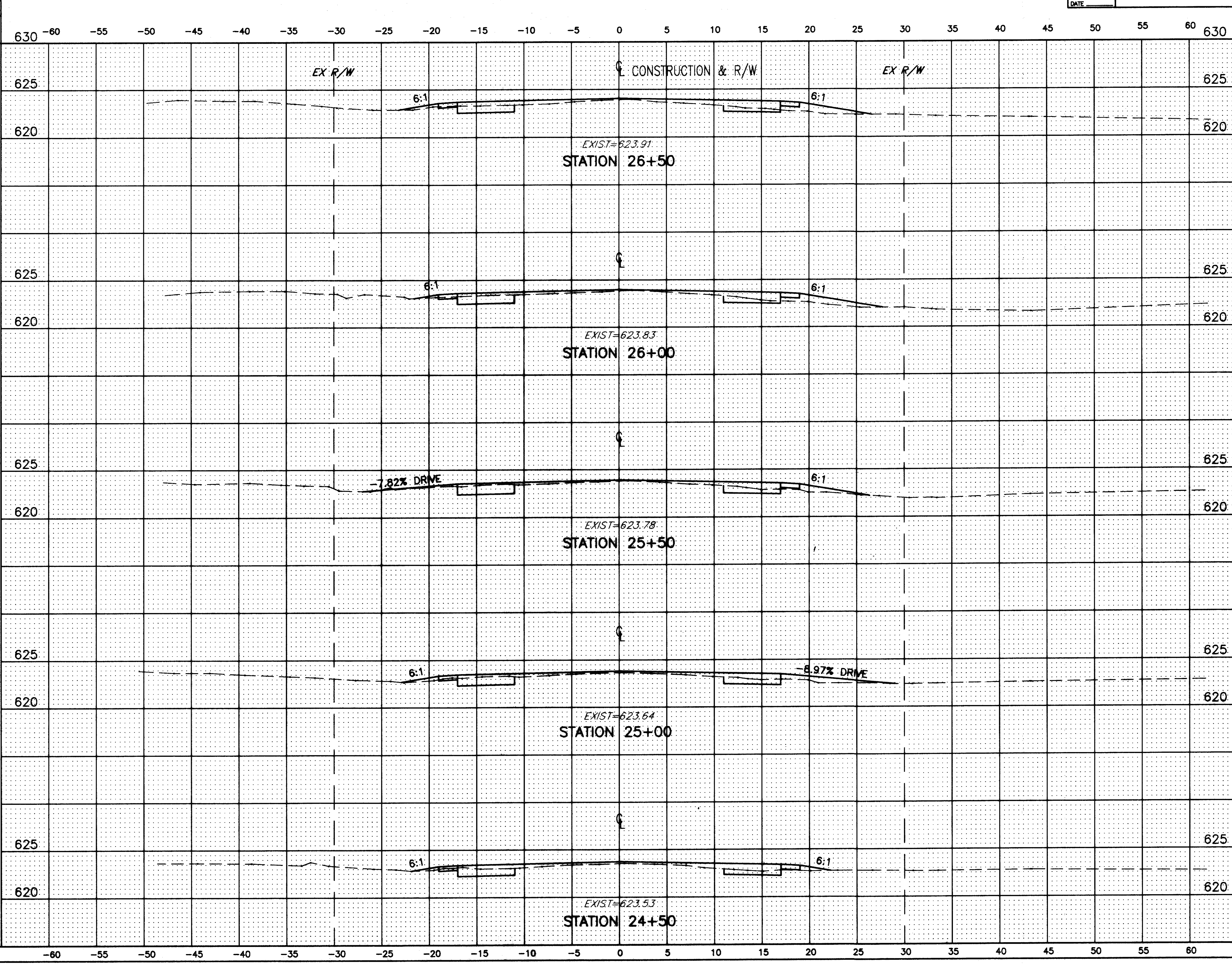
MUNSON ROAD CROSS-SECTIONS STA. 24+50 TO STA. 26+50
