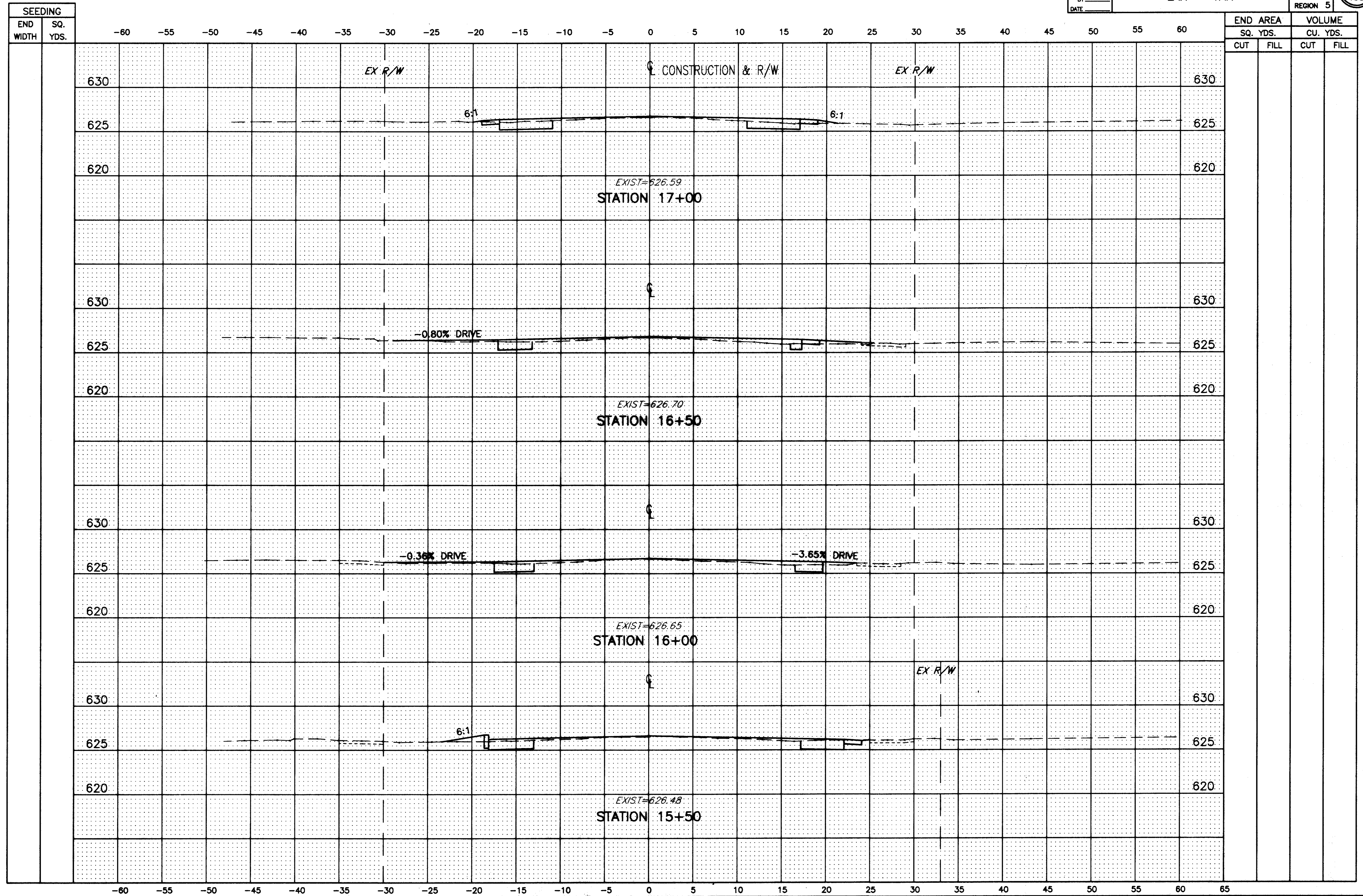
MUNSON ROAD CROSS-SECTIONS STA. 15+50 TO STA. 17+00
