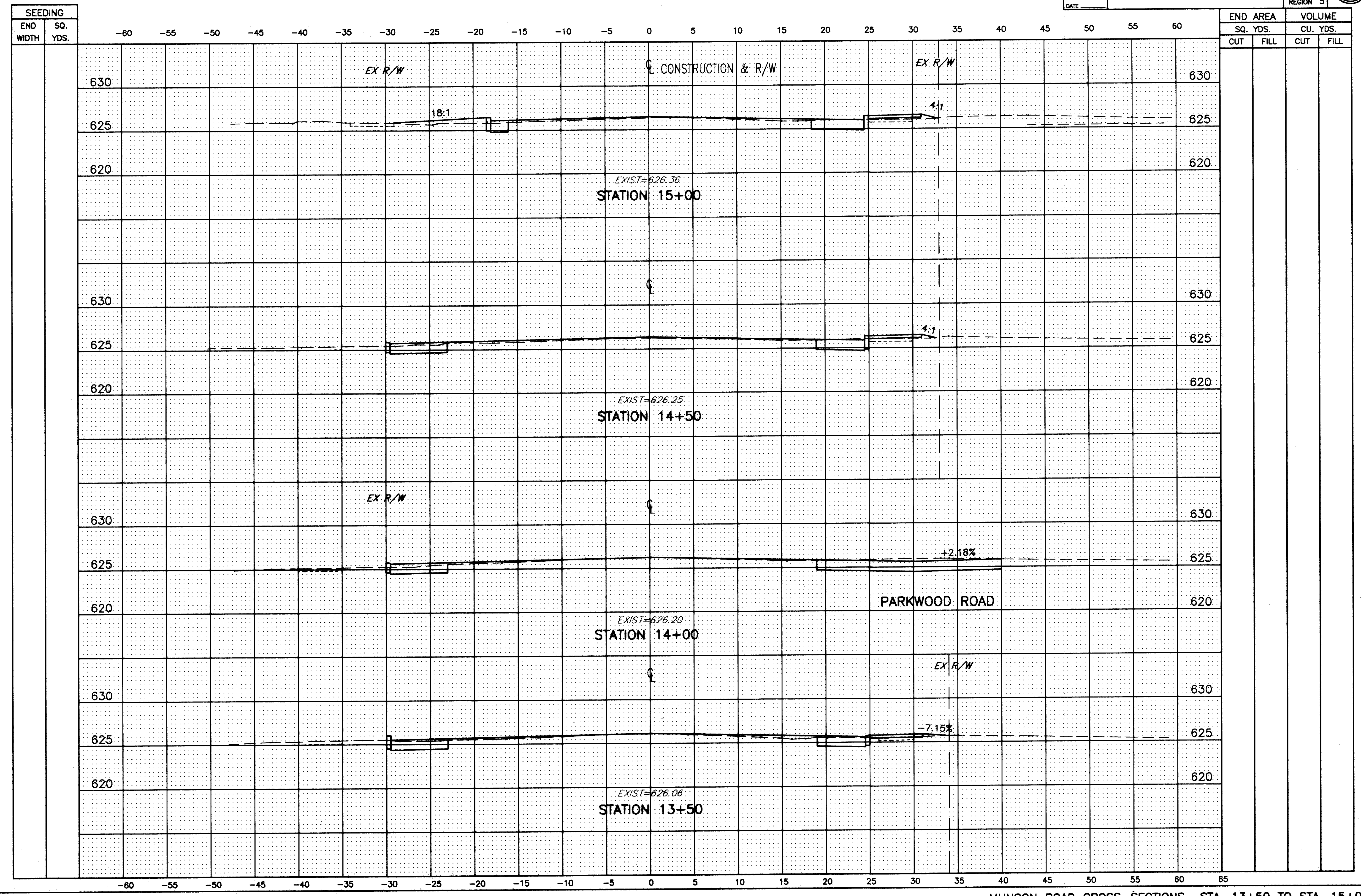
MUNSON ROAD CROSS-SECTIONS STA. 13+50 TO STA. 15+00
