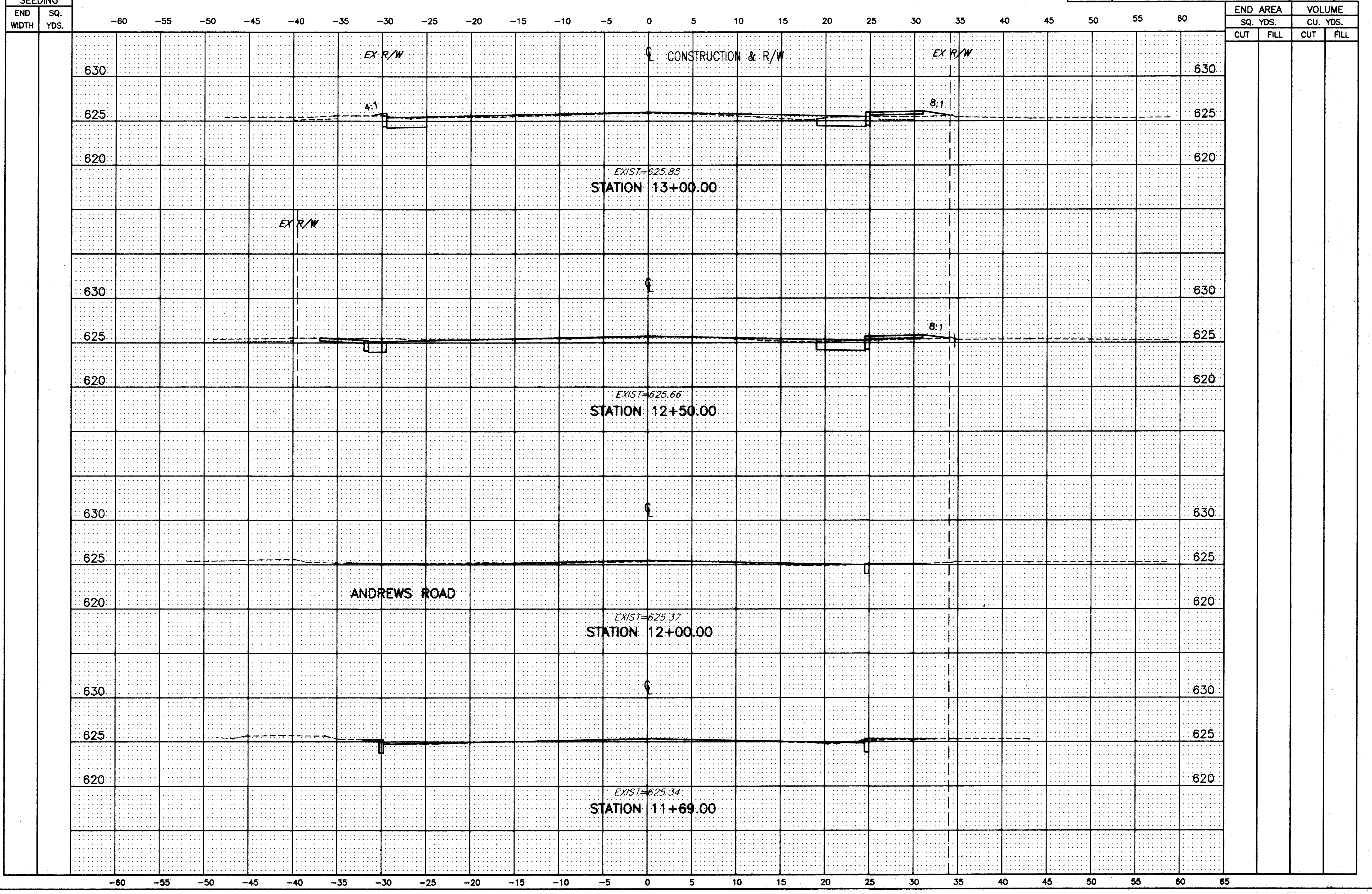
MUNSON ROAD CROSS-SECTIONS STA. 11+50 TO STA. 13+00
