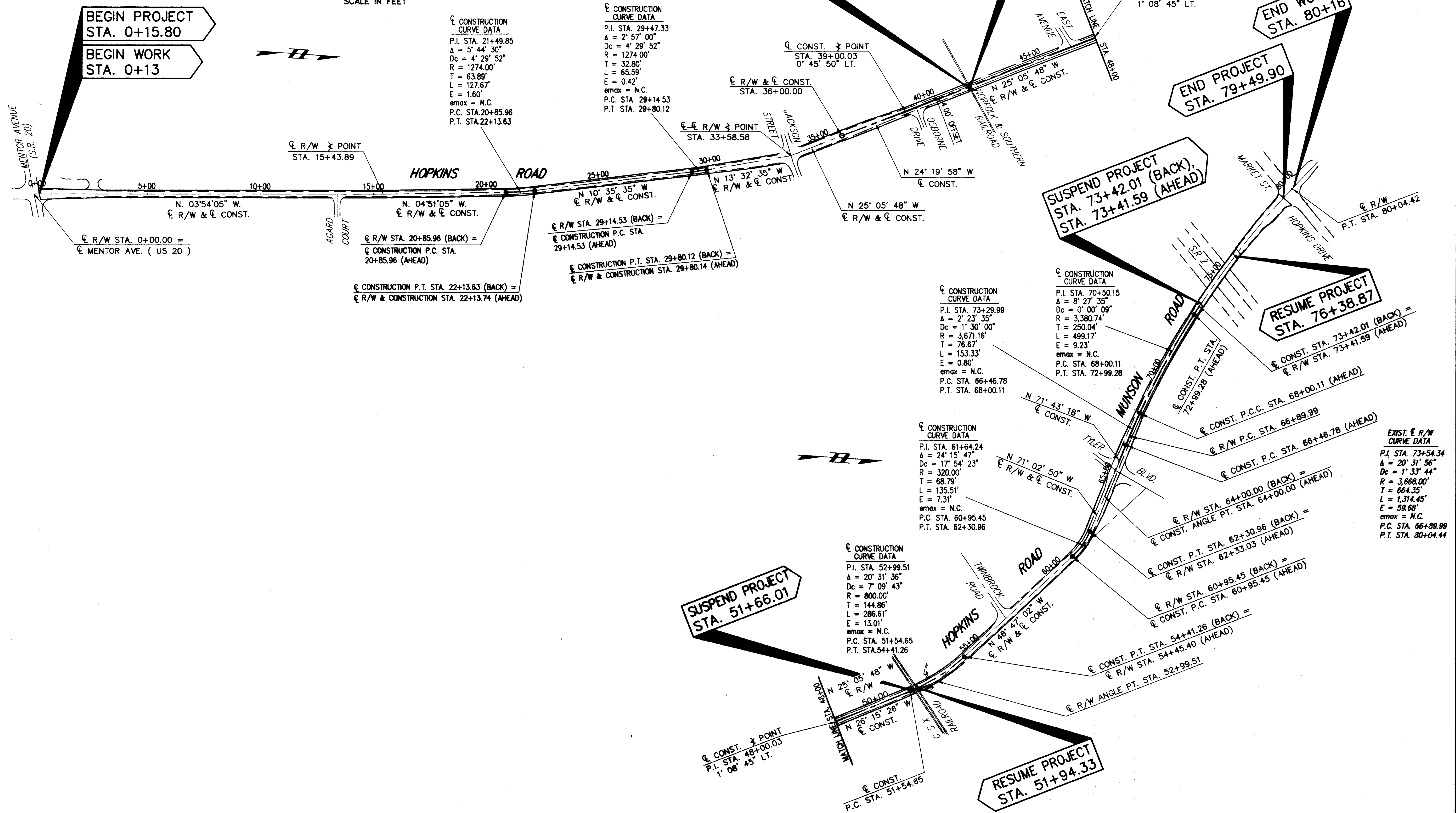
SCHEMATIC PLAN - HOPKINS/MUNSON ROAD
