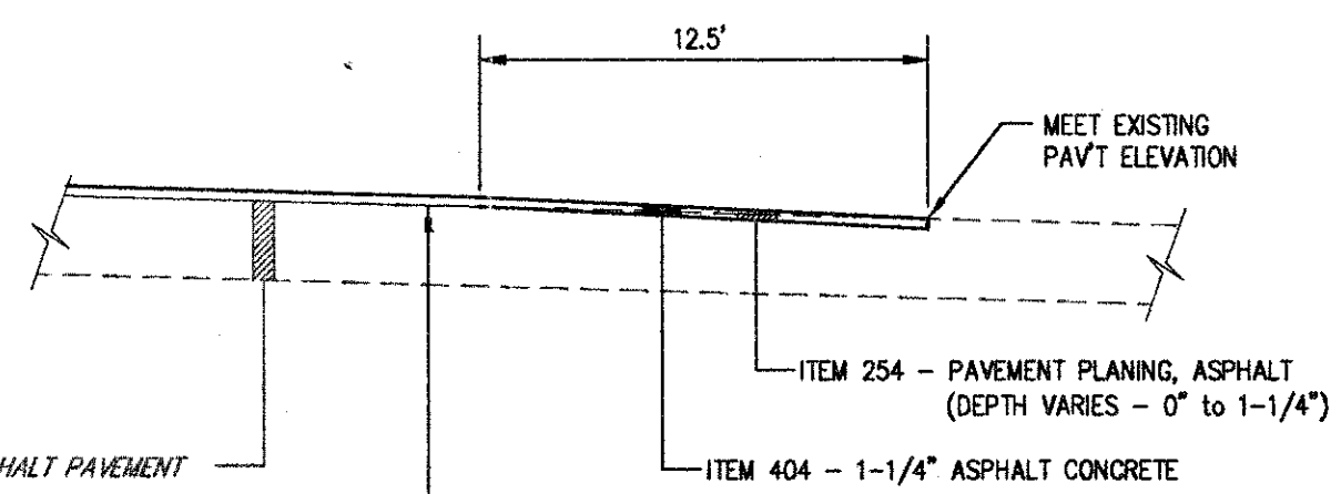
SECTION "C-C"
