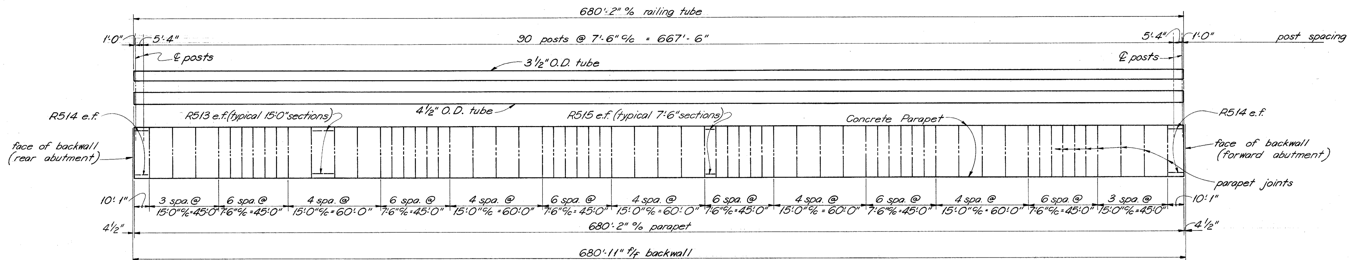
ELEVATION - WEST RAILING
