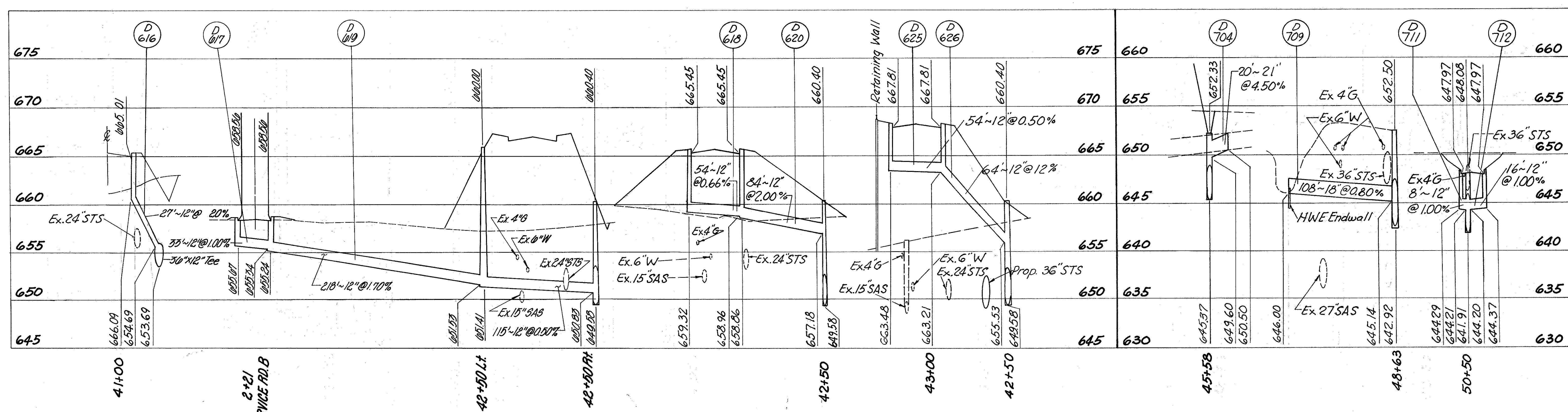
SEWER PROFILES
