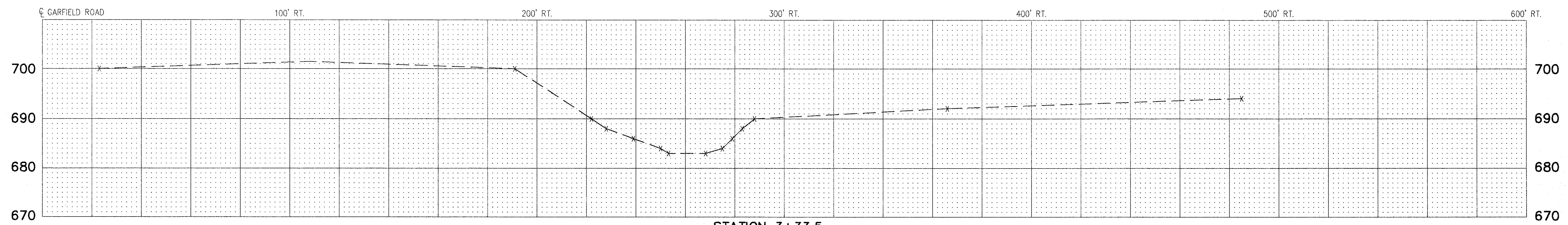
STATION 3+33.5
