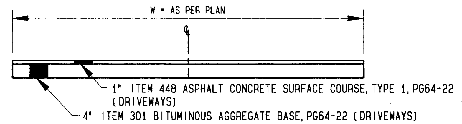
RESIDENTIAL ASPHALT DRIVE
