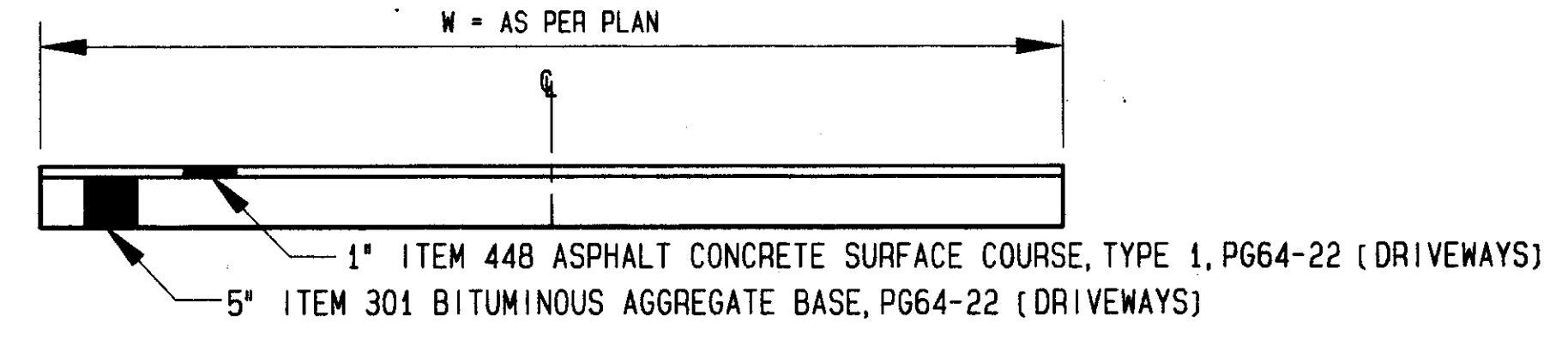
COMMERCIAL ASPHALT DRIVE
