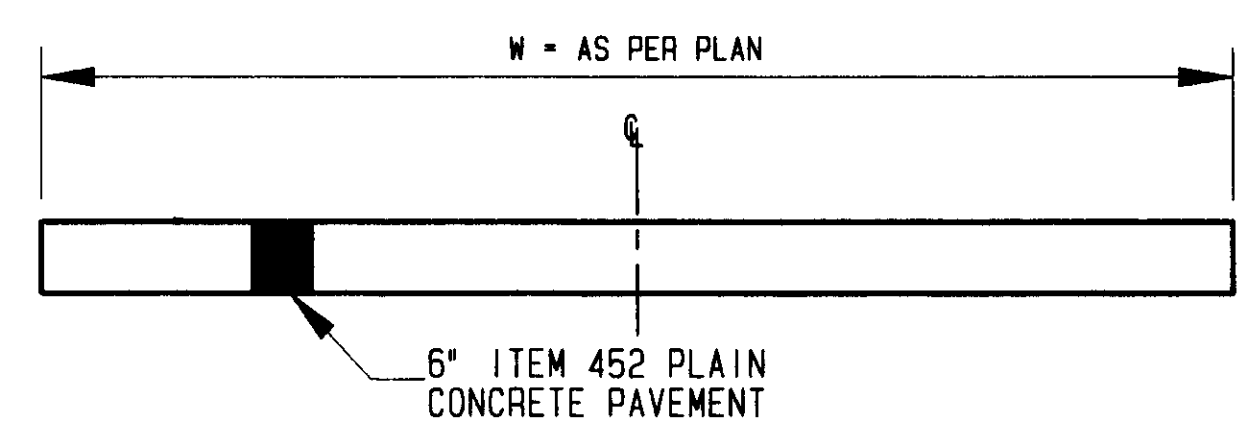
RESIDENTIAL CONCRETE DRIVE
