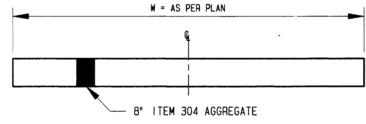
RESIDENTIAL STONE DRIVE
