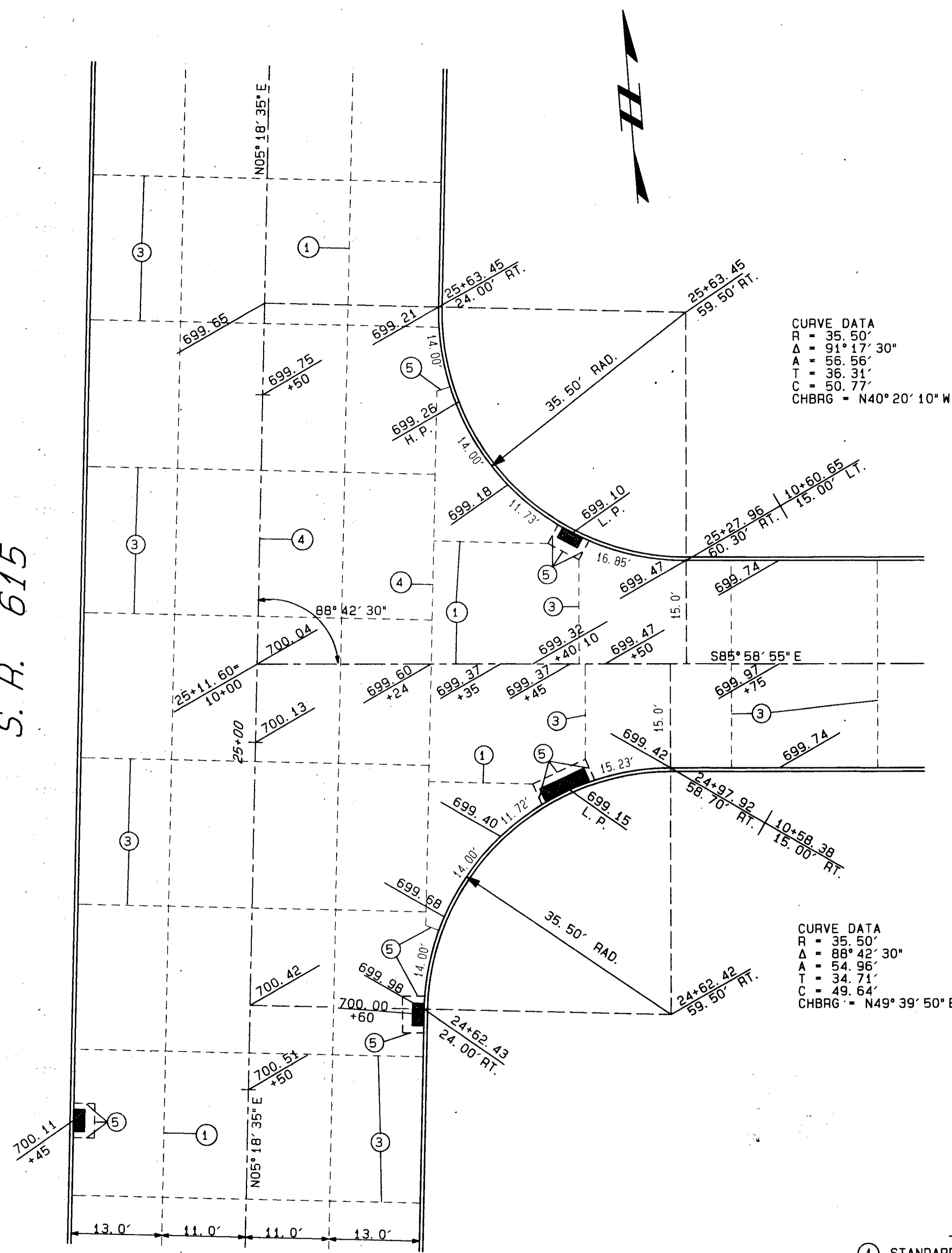
FORESTVIEW AVENUE (NOT TO SCALE)
