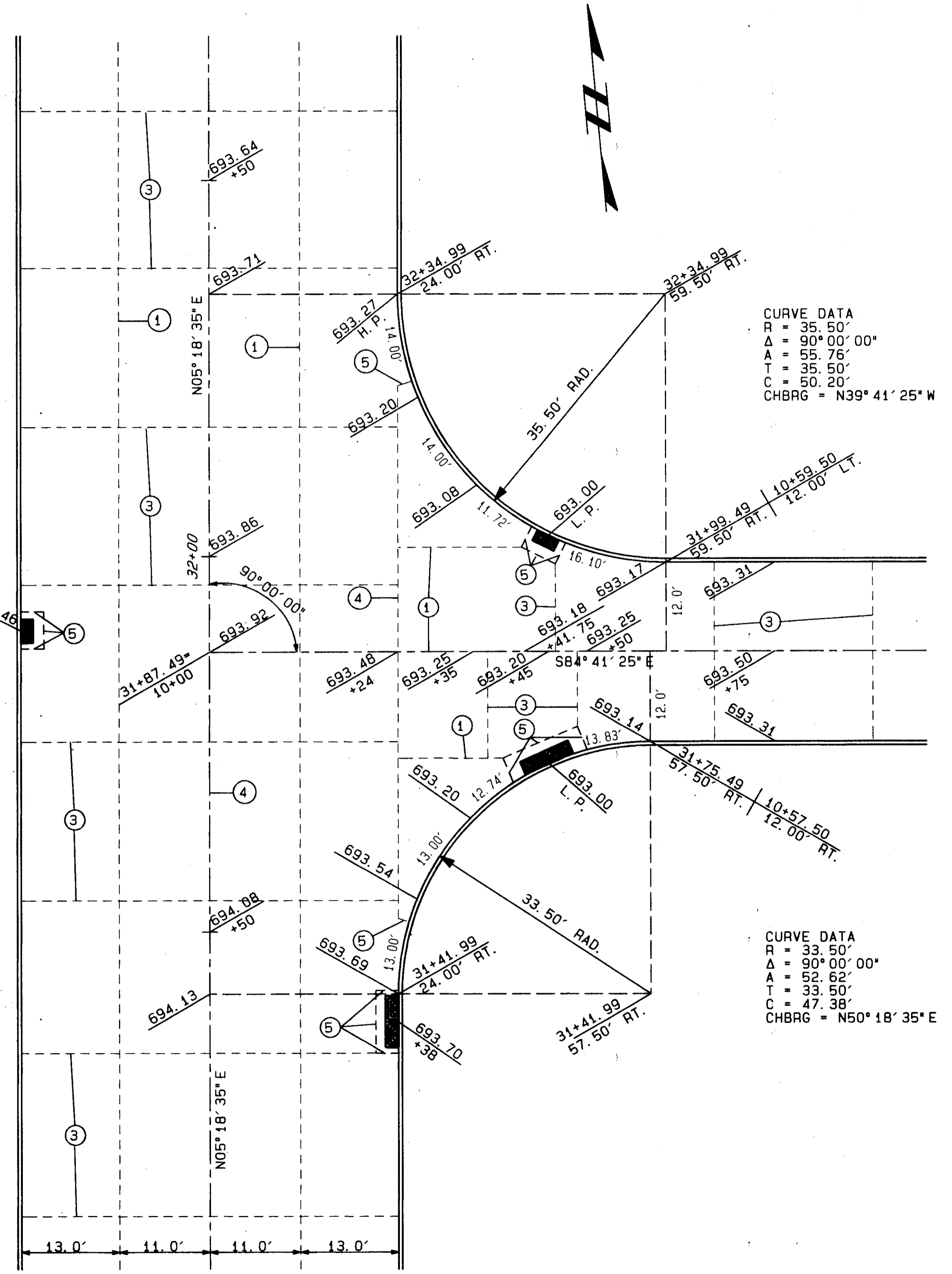
ESTHER STREET (NOT TO SCALE)
