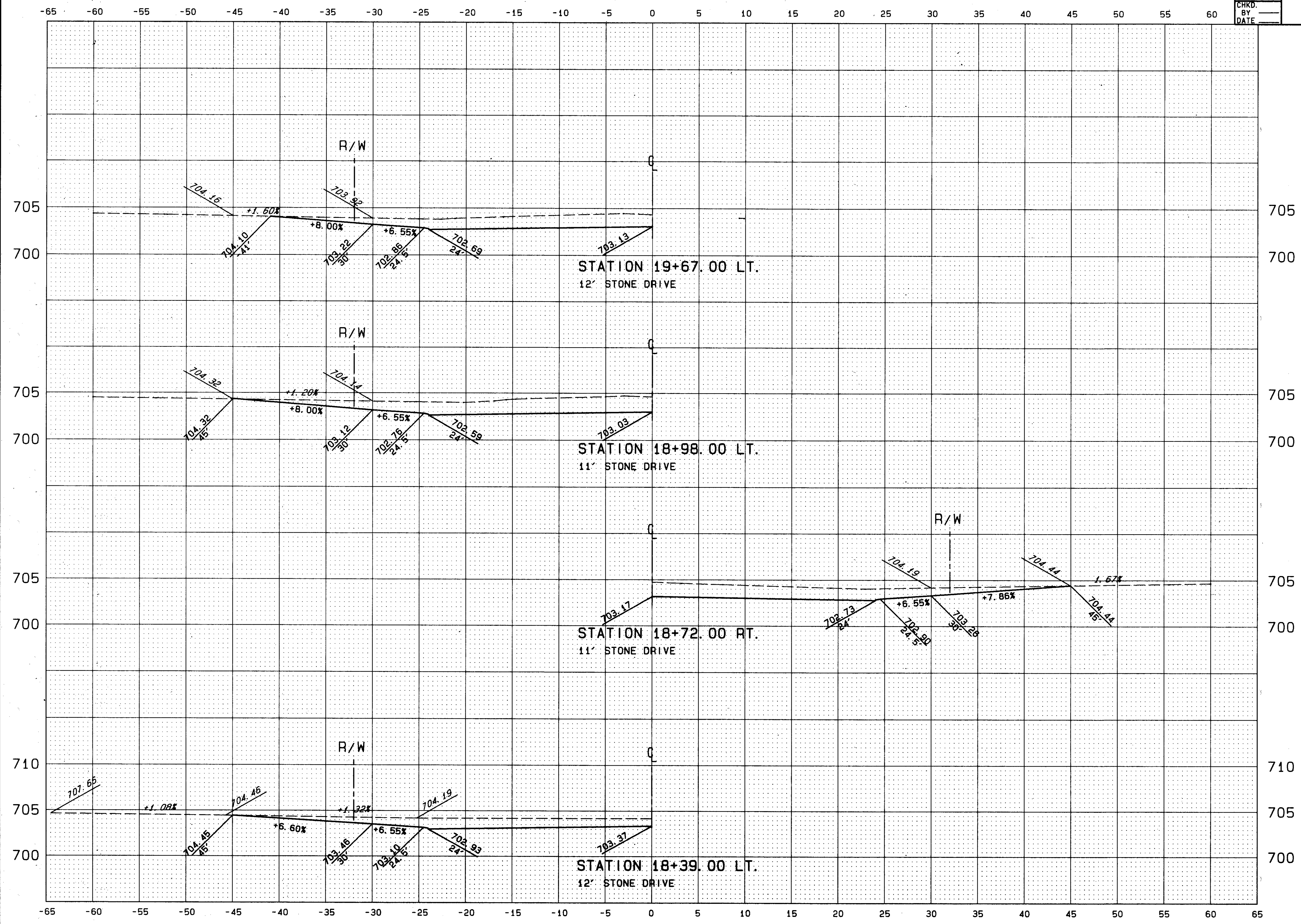
DRIVE PROFILES STA. 18+39 TO STA. 19+67
