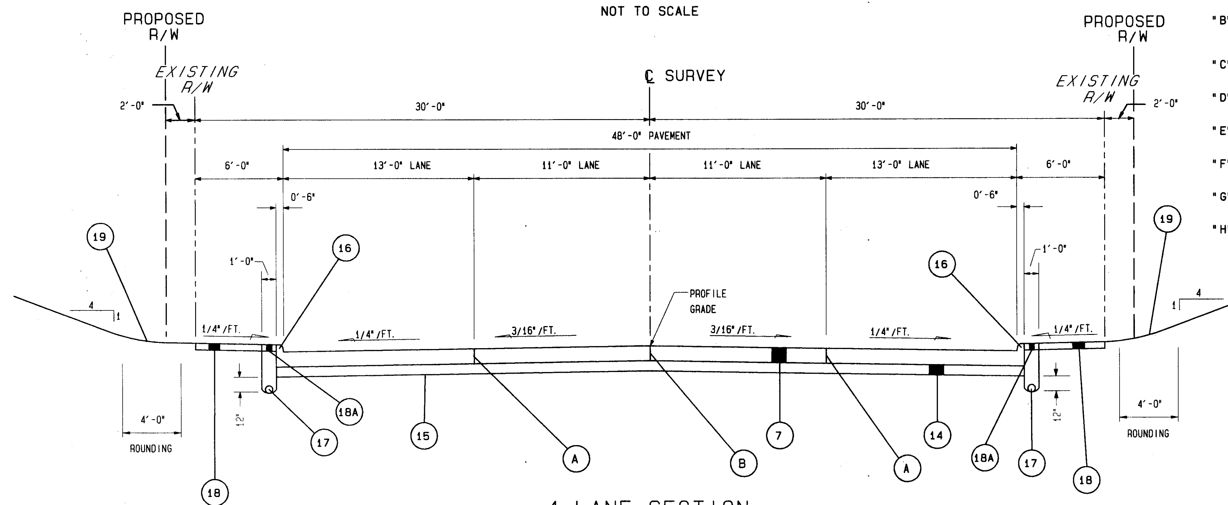
4 LANE SECTION
